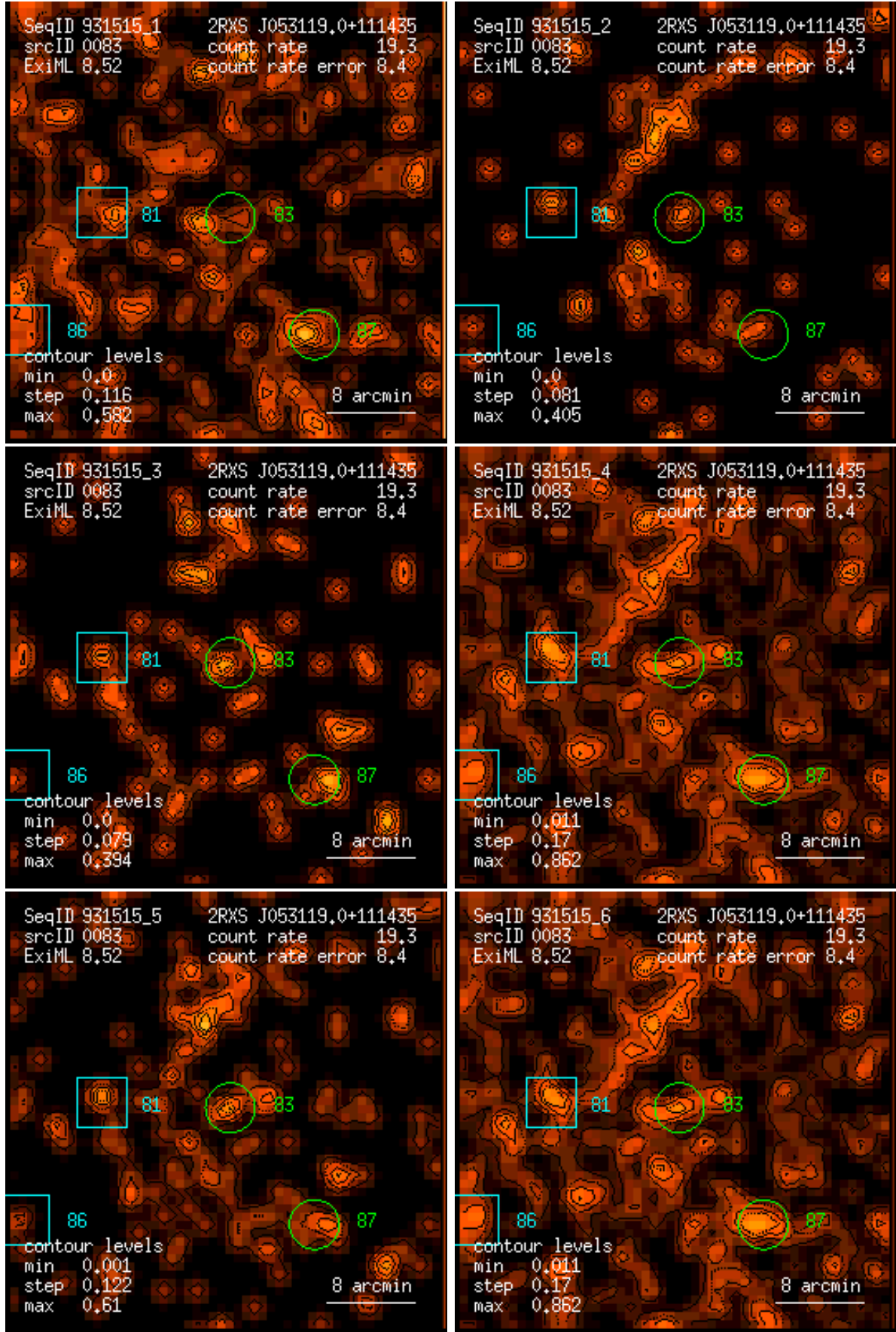
Figure 83: RASS 931515: detection 0083: band rate images, Gaussian filter: (1) PSPC channels 11 – 41, (2) 52 – 90, (3) 91 – 201, (4) 11 – 235, (5) 52 – 201, (6) 11 – 201. Broad band rates in counts/ks. Band rate contour levels in counts/ks/arcmin 2 .
