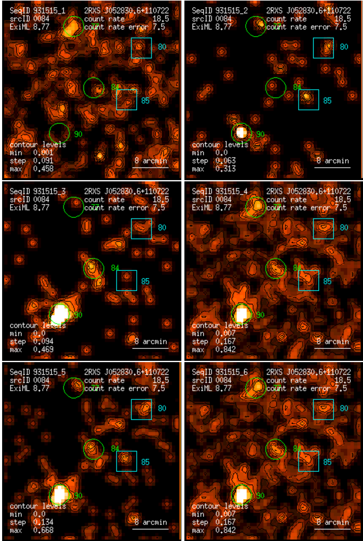
Figure 84: RASS 931515: detection 0084: band rate images, Gaussian filter: (1) PSPC channels 11 – 41, (2) 52 – 90, (3) 91 – 201, (4) 11 – 235, (5) 52 – 201, (6) 11 – 201. Broad band rates in counts/ks. Band rate contour levels in counts/ks/arcmin 2 .
