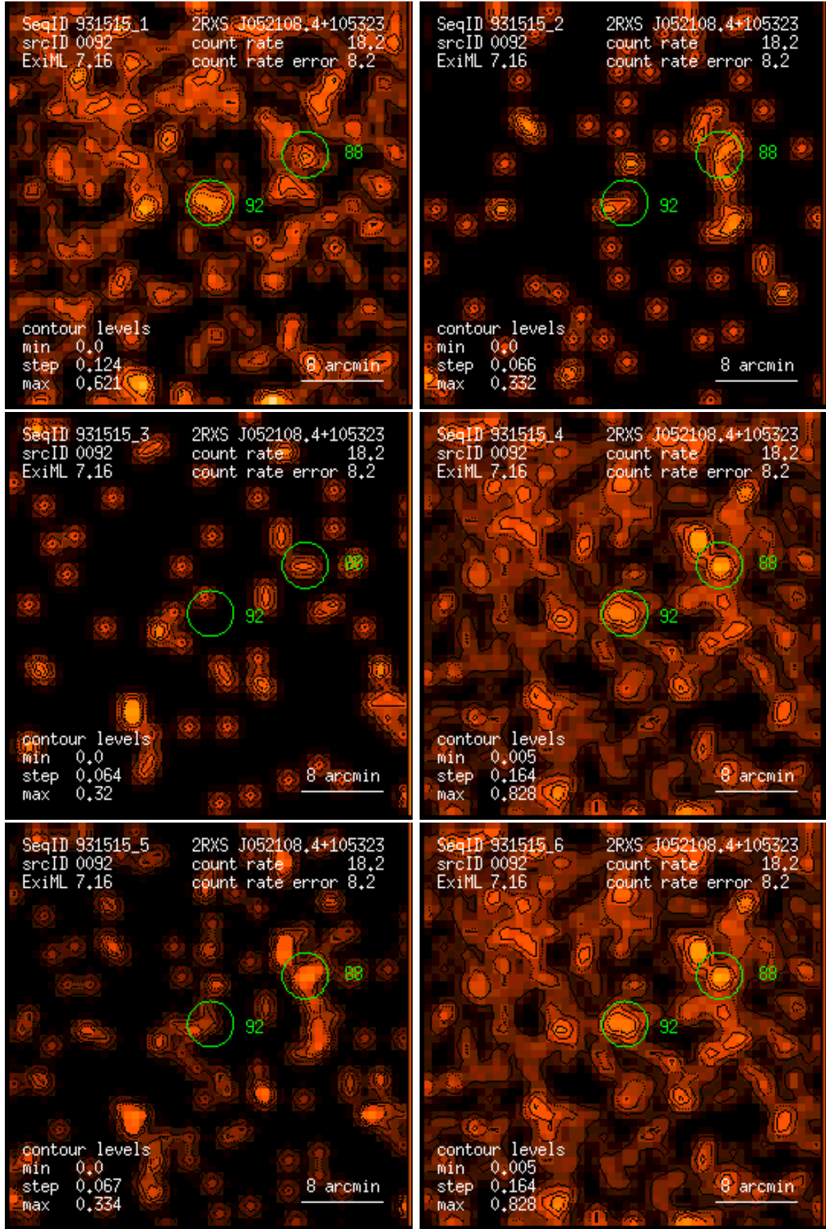
Figure 92: RASS 931515: detection 0092: band rate images, Gaussian filter: (1) PSPC channels 11 – 41, (2) 52 – 90, (3) 91 – 201, (4) 11 – 235, (5) 52 – 201, (6) 11 – 201. Broad band rates in counts/ks. Band rate contour levels in counts/ks/arcmin 2 .
