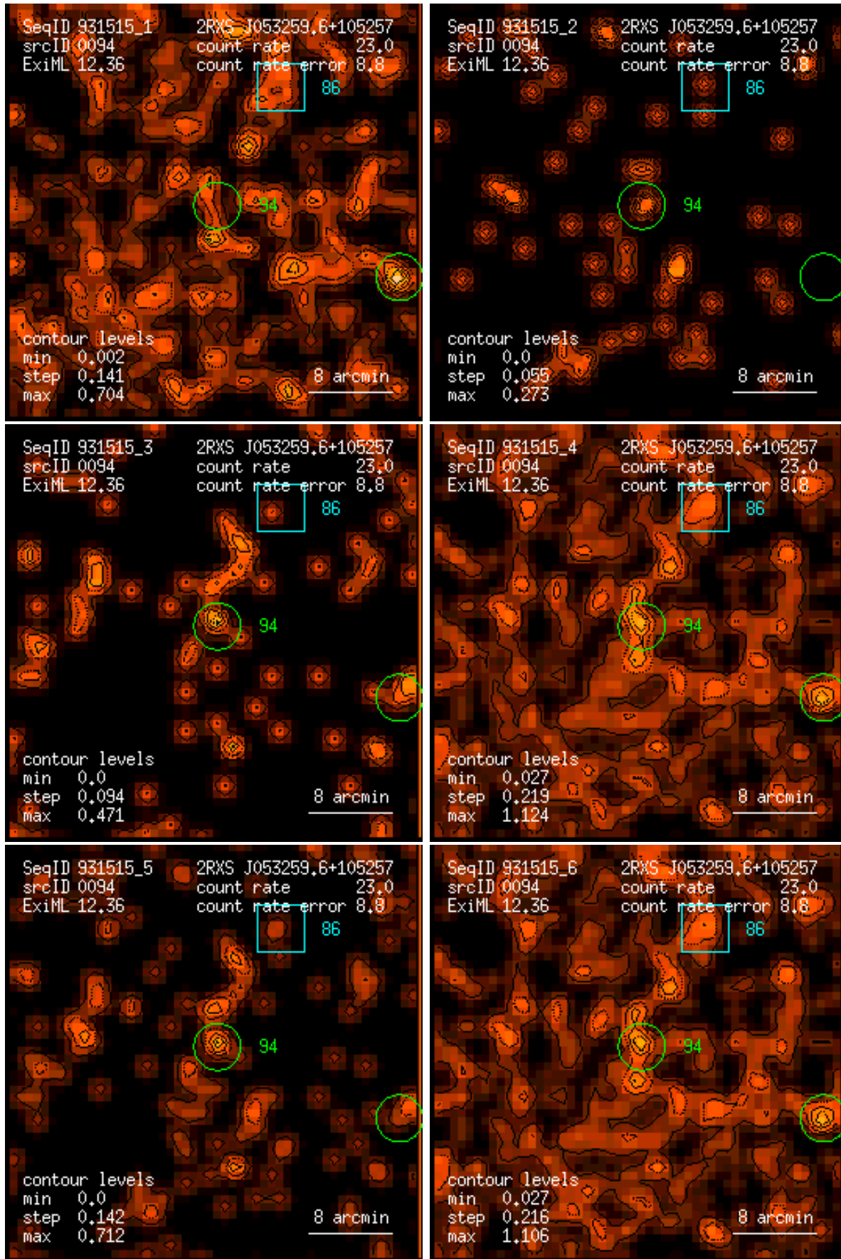
Figure 94: RASS 931515: detection 0094: band rate images, Gaussian filter: (1) PSPC channels 11 – 41, (2) 52 – 90, (3) 91 – 201, (4) 11 – 235, (5) 52 – 201, (6) 11 – 201. Broad band rates in counts/ks. Band rate contour levels in counts/ks/arcmin 2 .
