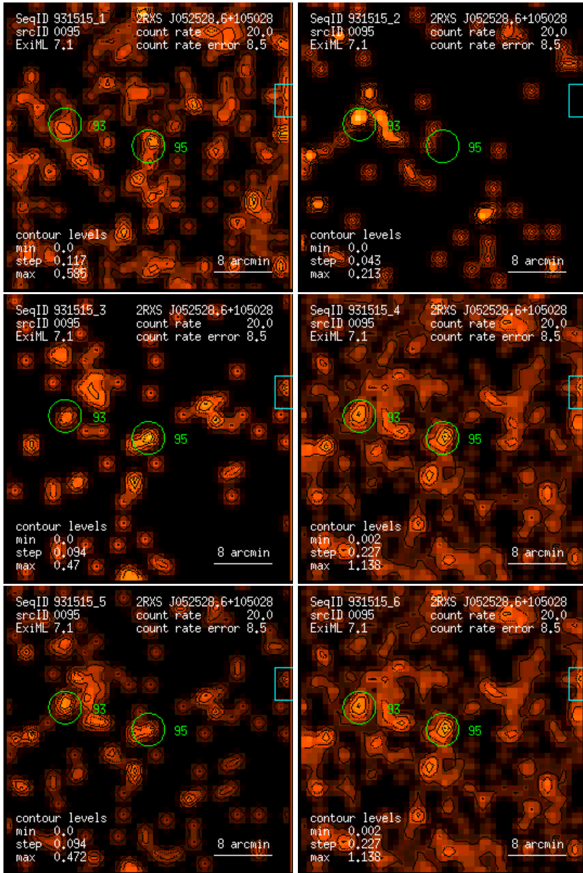
Figure 95: RASS 931515: detection 0095: band rate images, Gaussian filter: (1) PSPC channels 11 – 41, (2) 52 – 90, (3) 91 – 201, (4) 11 – 235, (5) 52 – 201, (6) 11 – 201. Broad band rates in counts/ks. Band rate contour levels in counts/ks/arcmin 2 .
