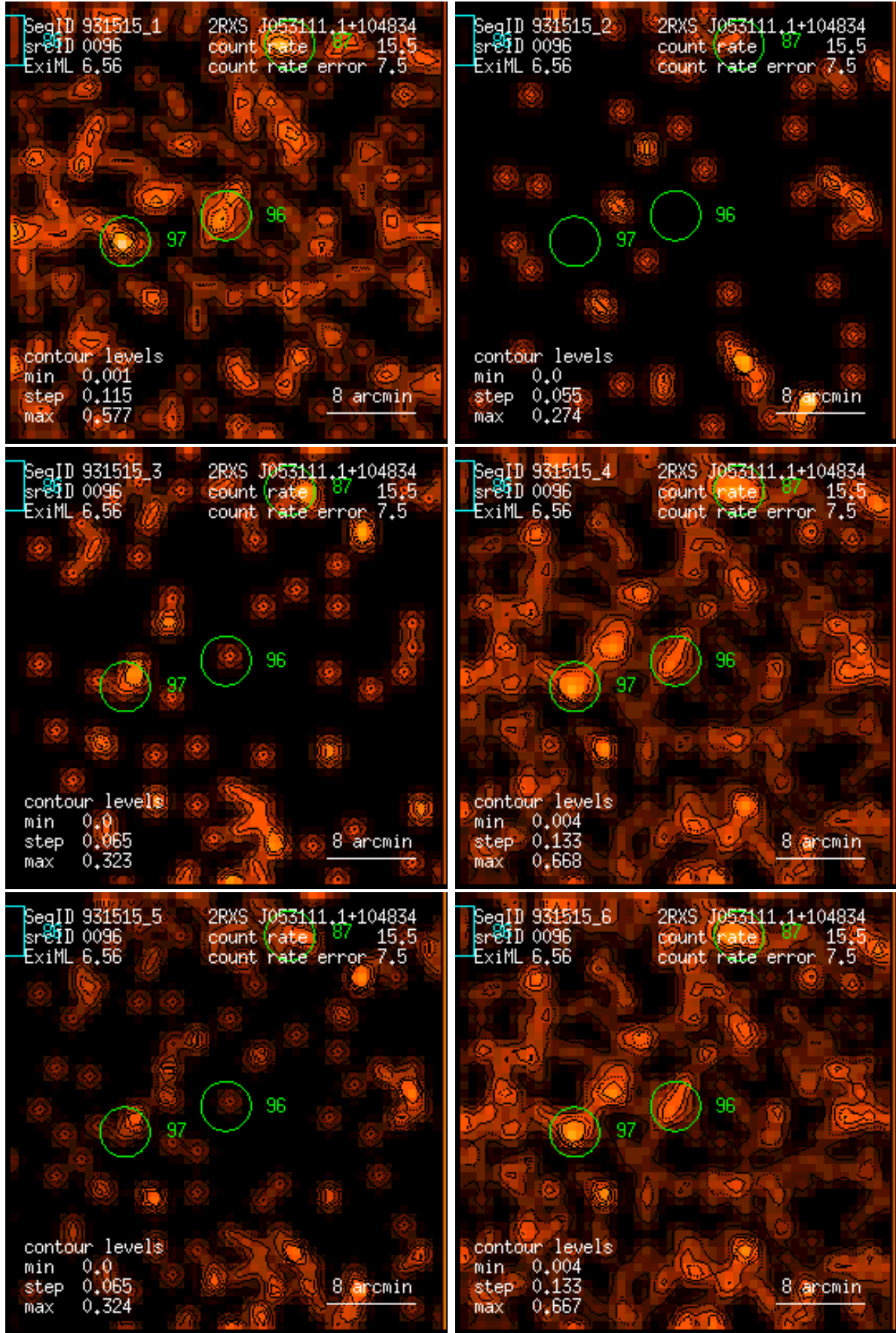
Figure 96: RASS 931515: detection 0096: band rate images, Gaussian filter: (1) PSPC channels 11 – 41, (2) 52 – 90, (3) 91 – 201, (4) 11 – 235, (5) 52 – 201, (6) 11 – 201. Broad band rates in counts/ks. Band rate contour levels in counts/ks/arcmin 2 .
