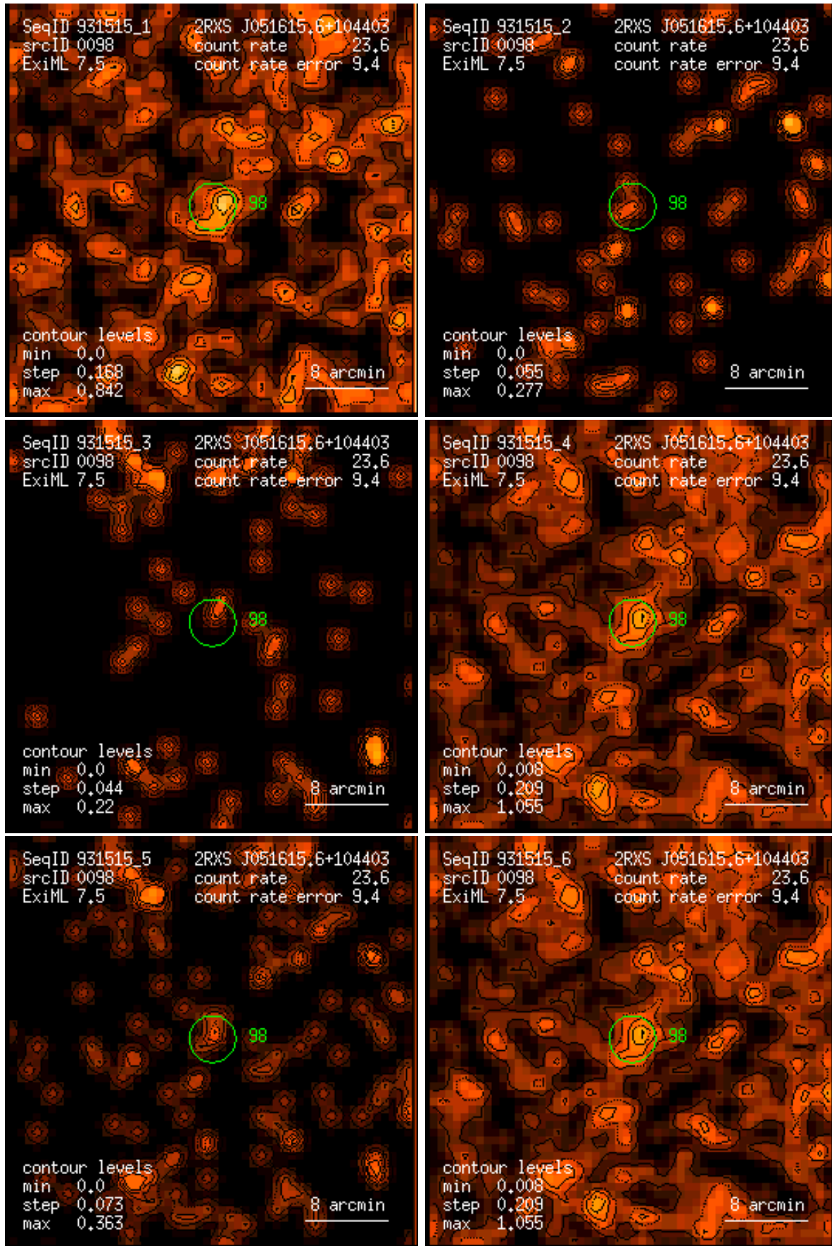
Figure 98: RASS 931515: detection 0098: band rate images, Gaussian filter: (1) PSPC channels 11 – 41, (2) 52 – 90, (3) 91 – 201, (4) 11 – 235, (5) 52 – 201, (6) 11 – 201. Broad band rates in counts/ks. Band rate contour levels in counts/ks/arcmin 2 .
