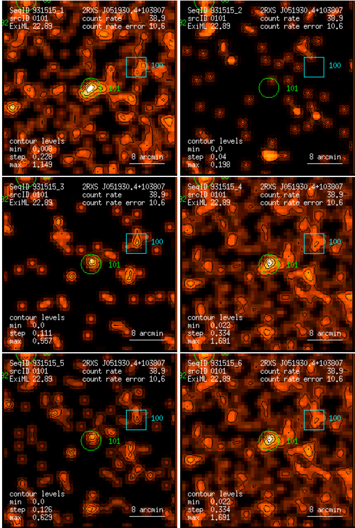
Figure 101: RASS 931515: detection 0101: band rate images, Gaussian filter: (1) PSPC channels 11 – 41, (2) 52 – 90, (3) 91 – 201, (4) 11 – 235, (5) 52 – 201, (6) 11 – 201. Broad band rates in counts/ks. Band rate contour levels in counts/ks/arcmin 2 .
