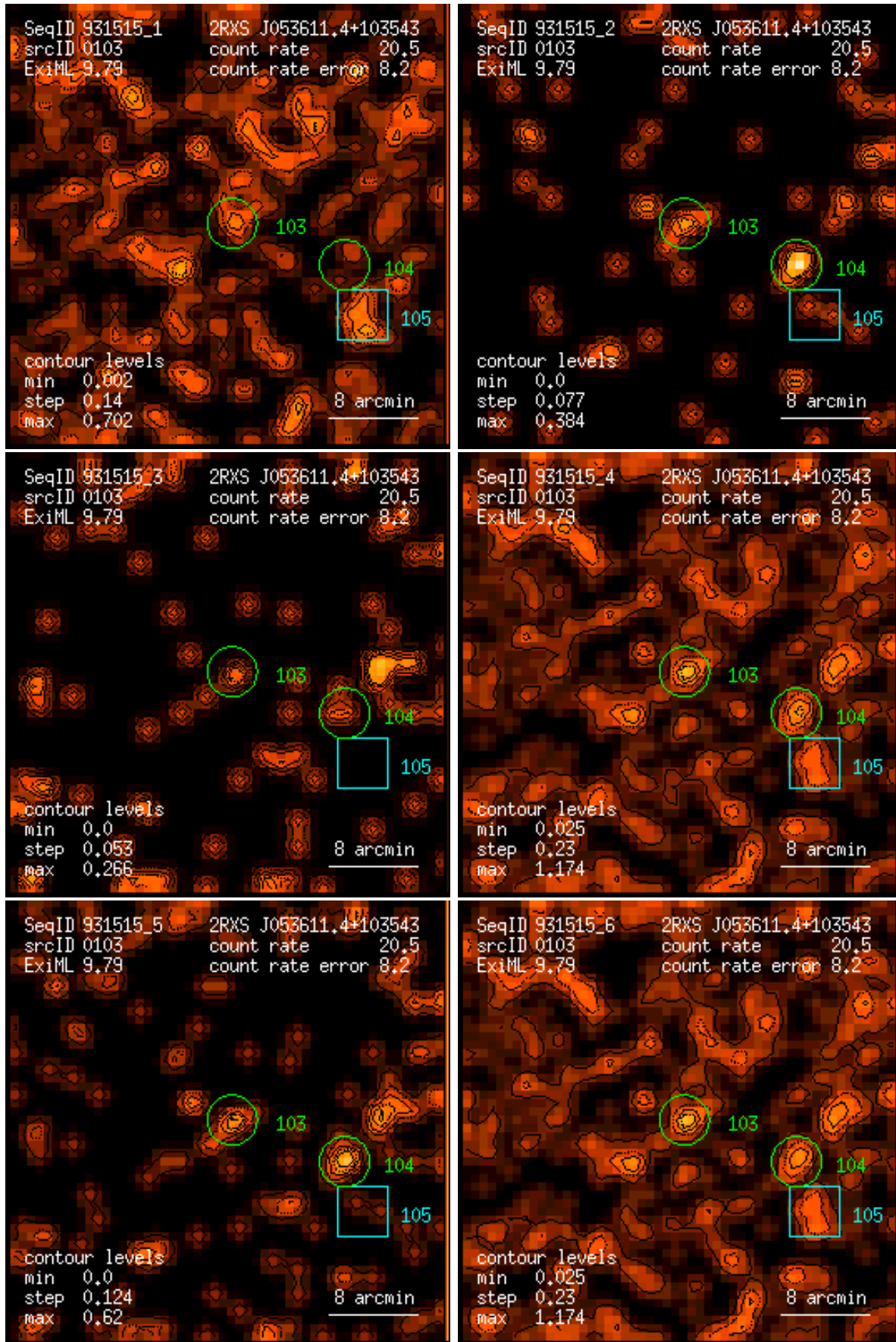
Figure 103: RASS 931515: detection 0103: band rate images, Gaussian filter: (1) PSPC channels 11 – 41, (2) 52 – 90, (3) 91 – 201, (4) 11 – 235, (5) 52 – 201, (6) 11 – 201. Broad band rates in counts/ks. Band rate contour levels in counts/ks/arcmin 2 .
