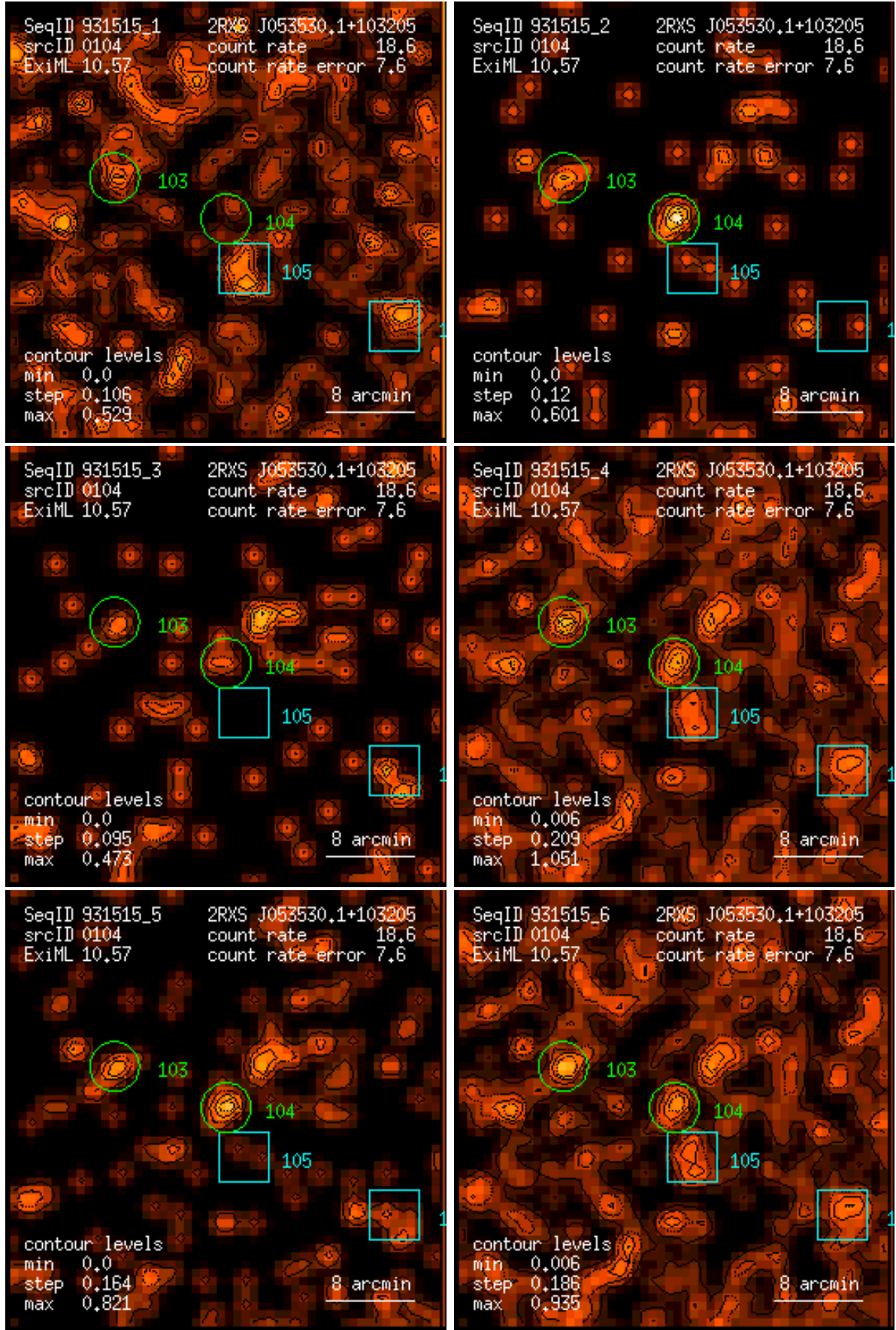
Figure 104: RASS 931515: detection 0104: band rate images, Gaussian filter: (1) PSPC channels 11 – 41, (2) 52 – 90, (3) 91 – 201, (4) 11 – 235, (5) 52 – 201, (6) 11 – 201. Broad band rates in counts/ks. Band rate contour levels in counts/ks/arcmin 2 .
