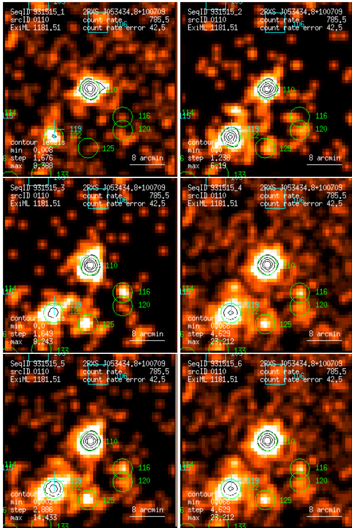
Figure 110: RASS 931515: detection 0110: band rate images, Gaussian filter: (1) PSPC channels 11 – 41, (2) 52 – 90, (3) 91 – 201, (4) 11 – 235, (5) 52 – 201, (6) 11 – 201. Broad band rates in counts/ks. Band rate contour levels in counts/ks/arcmin 2 .
