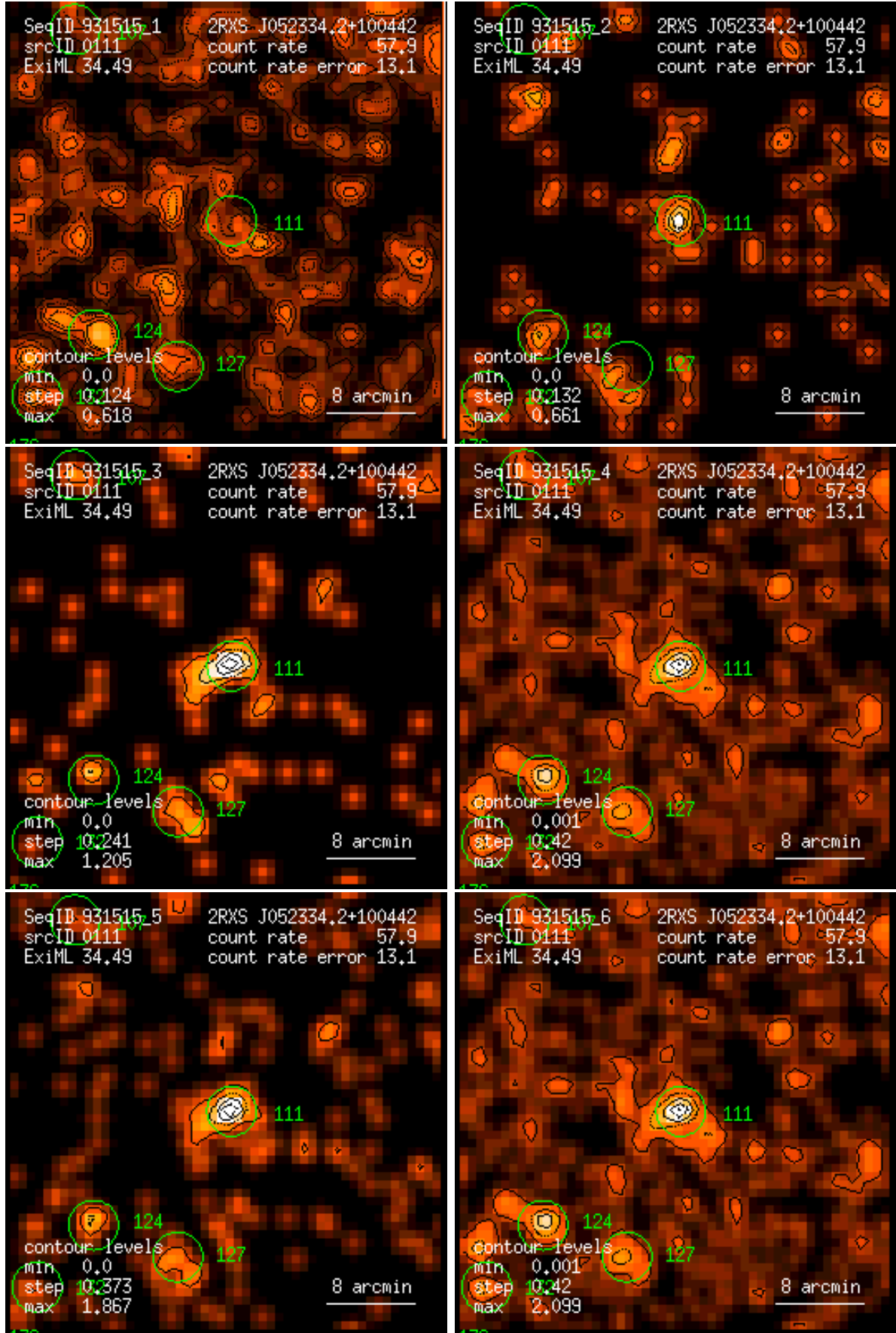
Figure 111: RASS 931515: detection 0111: band rate images, Gaussian filter: (1) PSPC channels 11 – 41, (2) 52 – 90, (3) 91 – 201, (4) 11 – 235, (5) 52 – 201, (6) 11 – 201. Broad band rates in counts/ks. Band rate contour levels in counts/ks/arcmin 2 .
