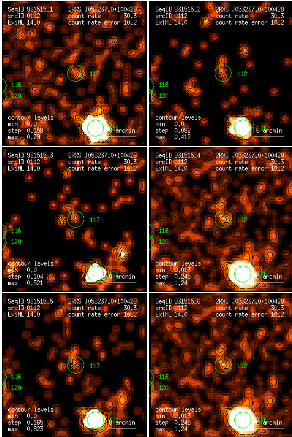
Figure 112: RASS 931515: detection 0112: band rate images, Gaussian filter: (1) PSPC channels 11 – 41, (2) 52 – 90, (3) 91 – 201, (4) 11 – 235, (5) 52 – 201, (6) 11 – 201. Broad band rates in counts/ks. Band rate contour levels in counts/ks/arcmin 2 .
