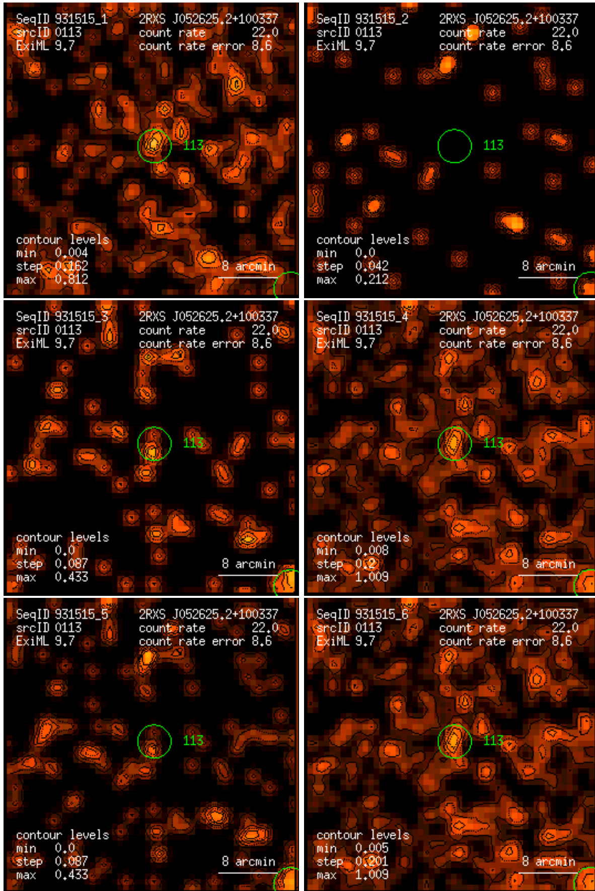
Figure 113: RASS 931515: detection 0113: band rate images, Gaussian filter: (1) PSPC channels 11 – 41, (2) 52 – 90, (3) 91 – 201, (4) 11 – 235, (5) 52 – 201, (6) 11 – 201. Broad band rates in counts/ks. Band rate contour levels in counts/ks/arcmin 2 .
