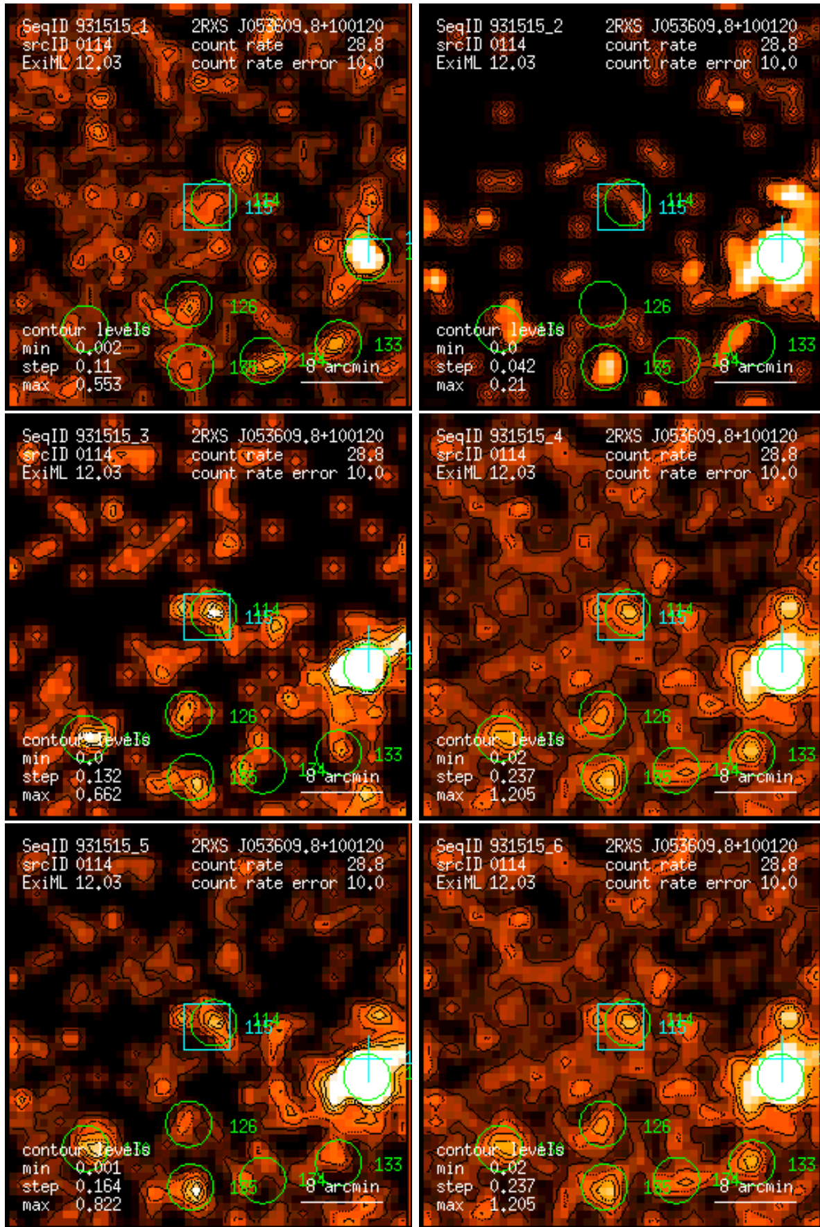
Figure 114: RASS 931515: detection 0114: band rate images, Gaussian filter: (1) PSPC channels 11 – 41, (2) 52 – 90, (3) 91 – 201, (4) 11 – 235, (5) 52 – 201, (6) 11 – 201. Broad band rates in counts/ks. Band rate contour levels in counts/ks/arcmin 2 .
