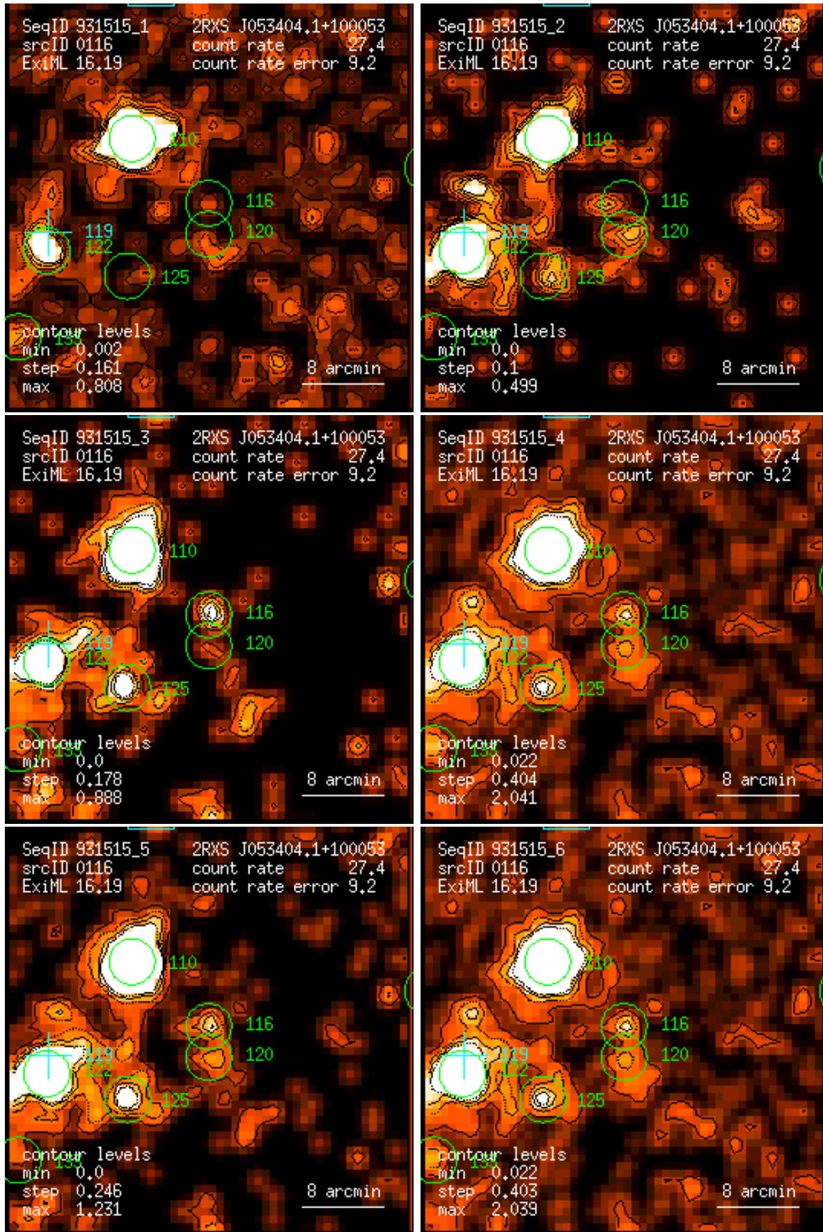
Figure 116: RASS 931515: detection 0116: band rate images, Gaussian filter: (1) PSPC channels 11 – 41, (2) 52 – 90, (3) 91 – 201, (4) 11 – 235, (5) 52 – 201, (6) 11 – 201. Broad band rates in counts/ks. Band rate contour levels in counts/ks/arcmin 2 .
