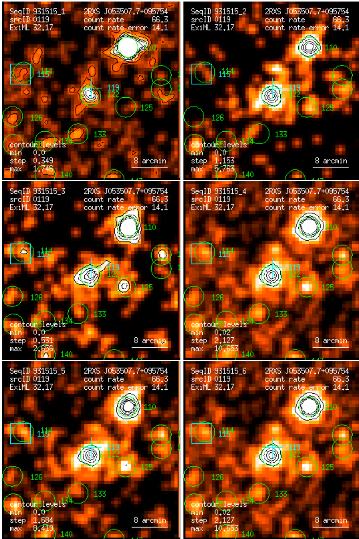
Figure 119: RASS 931515: detection 0119: band rate images, Gaussian filter: (1) PSPC channels 11 – 41, (2) 52 – 90, (3) 91 – 201, (4) 11 – 235, (5) 52 – 201, (6) 11 – 201. Broad band rates in counts/ks. Band rate contour levels in counts/ks/arcmin 2 .
