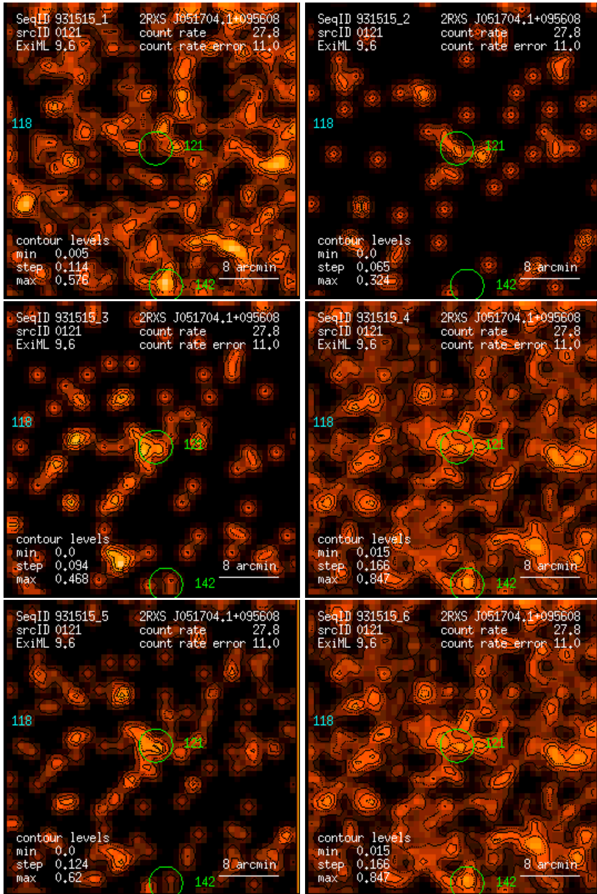
Figure 121: RASS 931515: detection 0121: band rate images, Gaussian filter: (1) PSPC channels 11 – 41, (2) 52 – 90, (3) 91 – 201, (4) 11 – 235, (5) 52 – 201, (6) 11 – 201. Broad band rates in counts/ks. Band rate contour levels in counts/ks/arcmin 2 .
