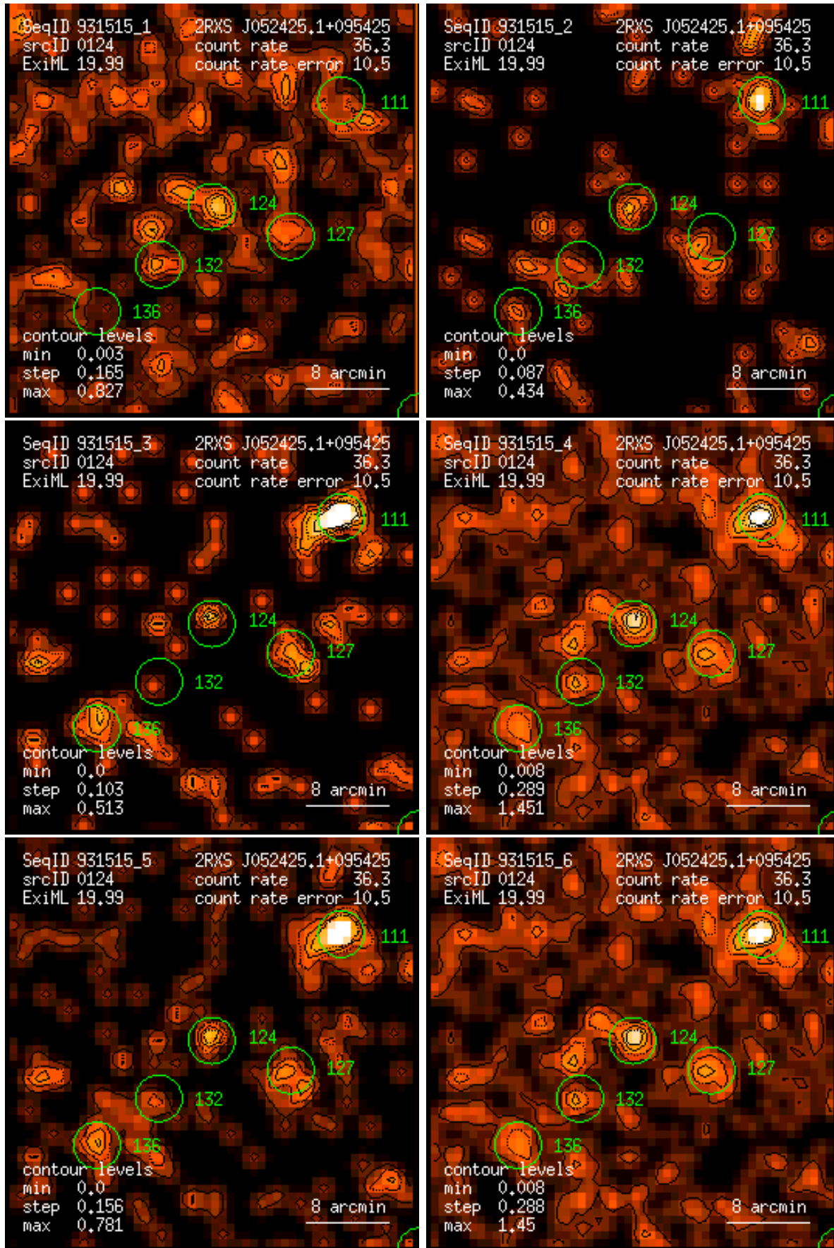
Figure 124: RASS 931515: detection 0124: band rate images, Gaussian filter: (1) PSPC channels 11 – 41, (2) 52 – 90, (3) 91 – 201, (4) 11 – 235, (5) 52 – 201, (6) 11 – 201. Broad band rates in counts/ks. Band rate contour levels in counts/ks/arcmin 2 .
