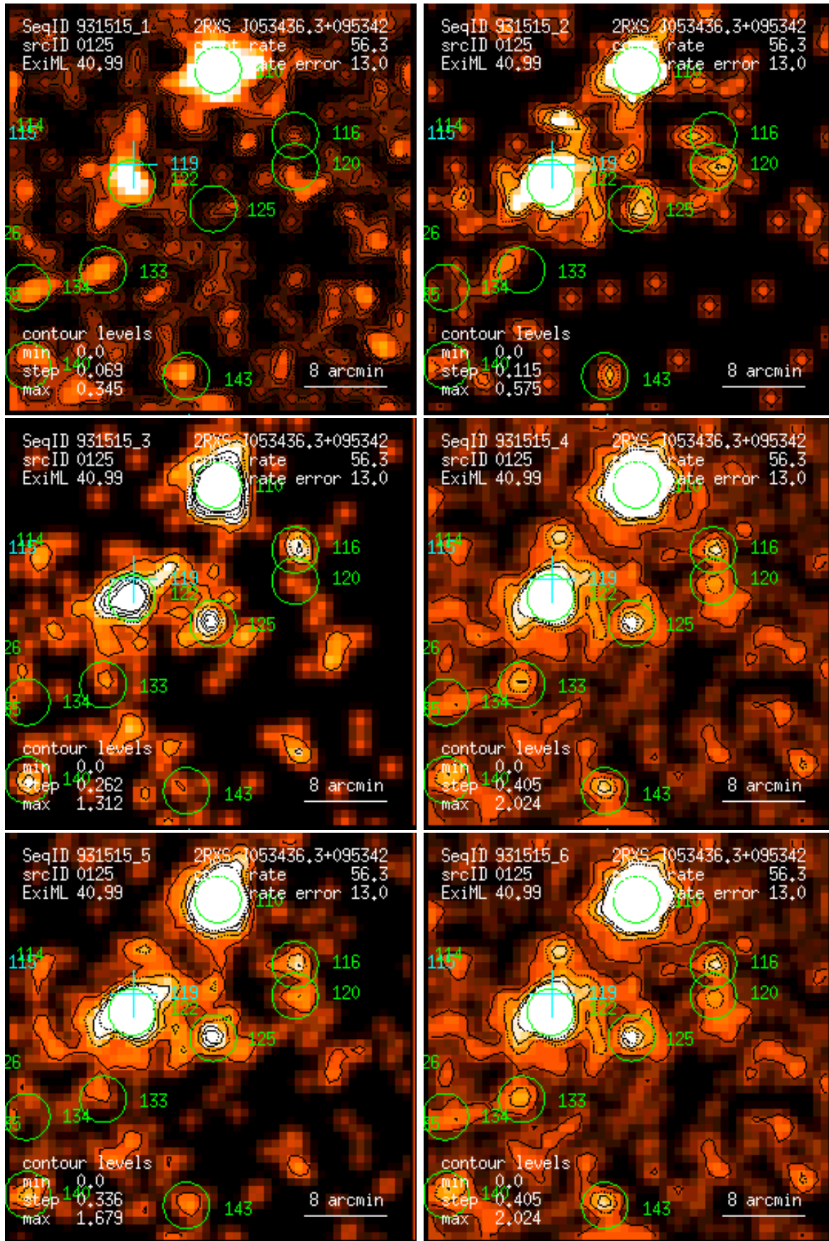
Figure 125: RASS 931515: detection 0125: band rate images, Gaussian filter: (1) PSPC channels 11 – 41, (2) 52 – 90, (3) 91 – 201, (4) 11 – 235, (5) 52 – 201, (6) 11 – 201. Broad band rates in counts/ks. Band rate contour levels in counts/ks/arcmin 2 .
