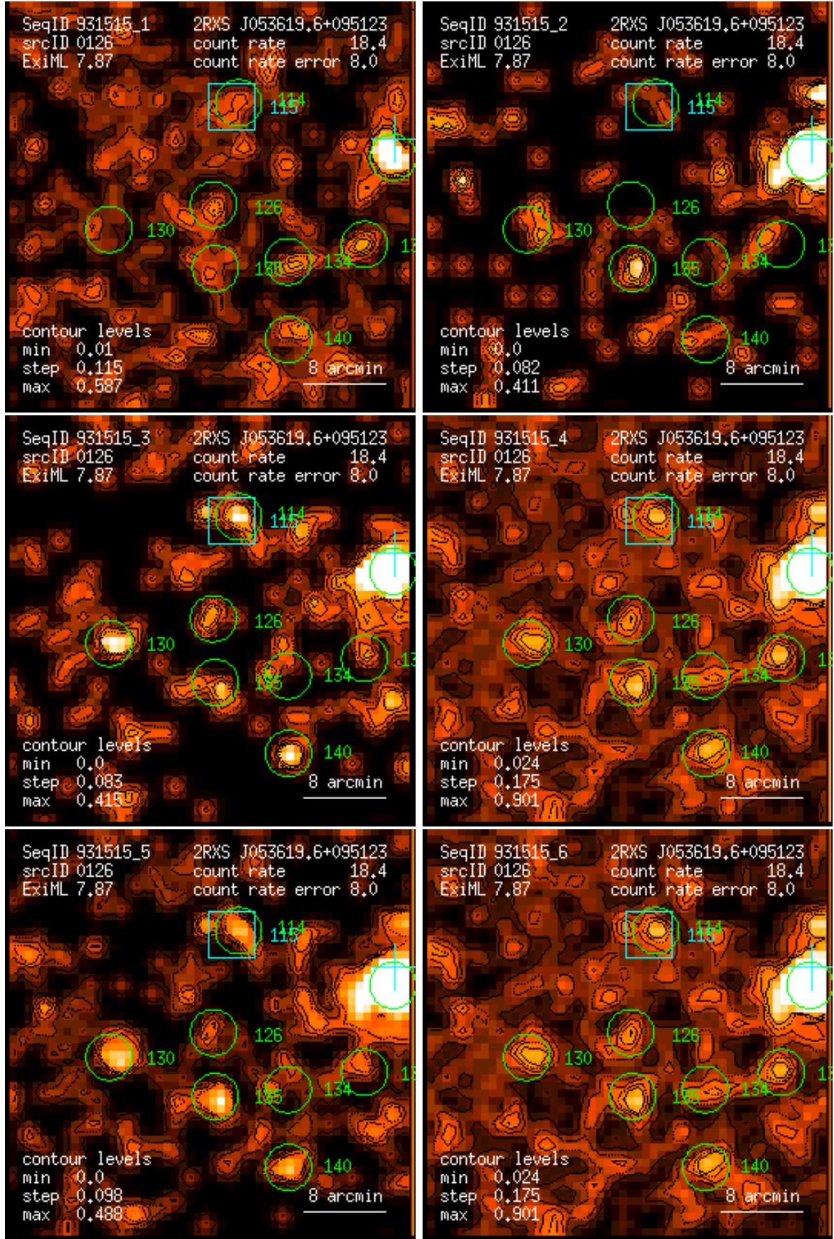
Figure 126: RASS 931515: detection 0126: band rate images, Gaussian filter: (1) PSPC channels 11 – 41, (2) 52 – 90, (3) 91 – 201, (4) 11 – 235, (5) 52 – 201, (6) 11 – 201. Broad band rates in counts/ks. Band rate contour levels in counts/ks/arcmin 2 .
