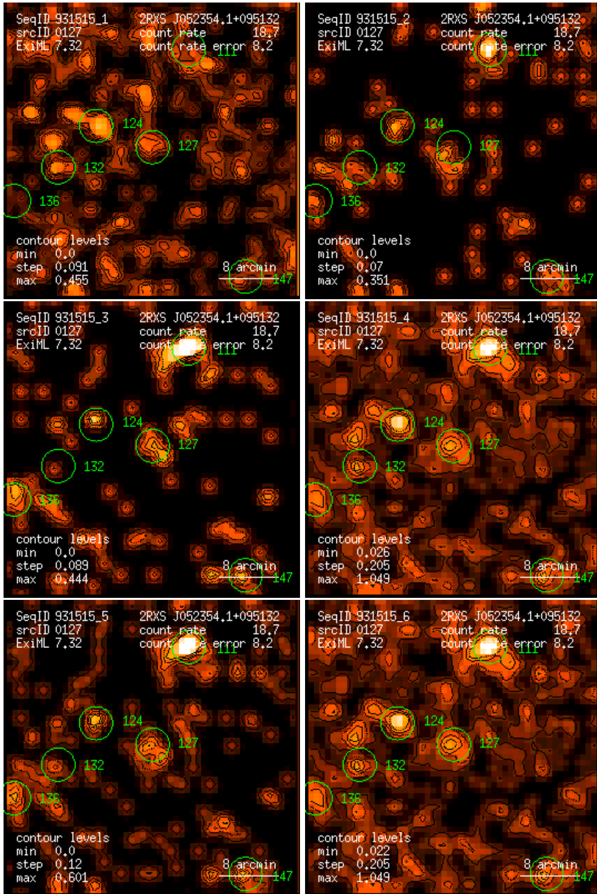
Figure 127: RASS 931515: detection 0127: band rate images, Gaussian filter: (1) PSPC channels 11 – 41, (2) 52 – 90, (3) 91 – 201, (4) 11 – 235, (5) 52 – 201, (6) 11 – 201. Broad band rates in counts/ks. Band rate contour levels in counts/ks/arcmin 2 .
