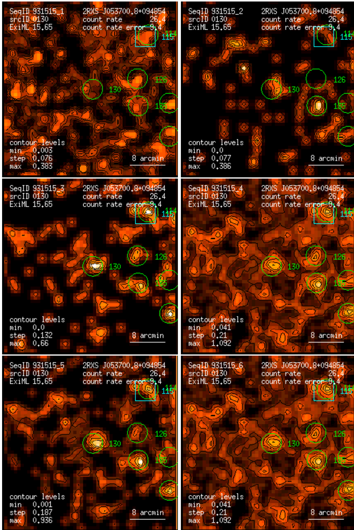
Figure 130: RASS 931515: detection 0130: band rate images, Gaussian filter: (1) PSPC channels 11 – 41, (2) 52 – 90, (3) 91 – 201, (4) 11 – 235, (5) 52 – 201, (6) 11 – 201. Broad band rates in counts/ks. Band rate contour levels in counts/ks/arcmin 2 .
