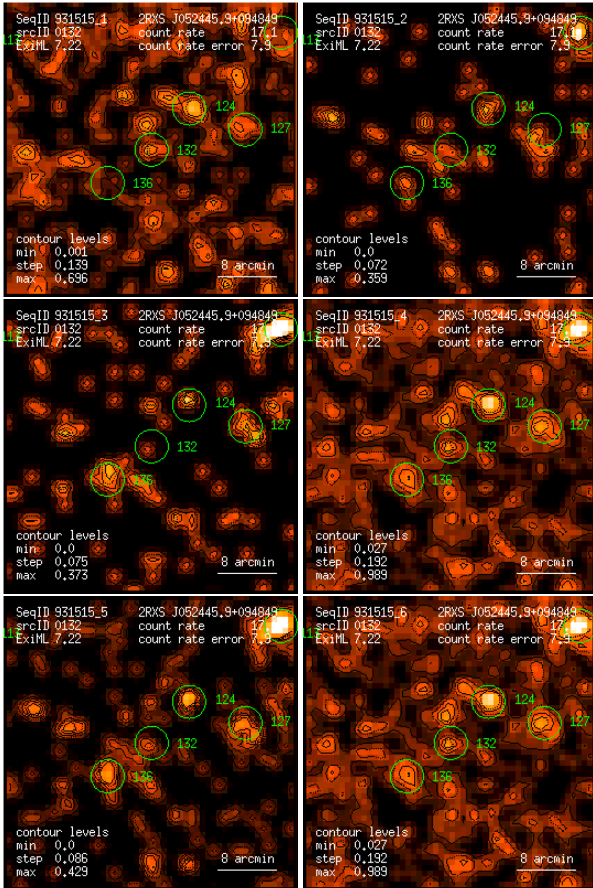
Figure 132: RASS 931515: detection 0132: band rate images, Gaussian filter: (1) PSPC channels 11 – 41, (2) 52 – 90, (3) 91 – 201, (4) 11 – 235, (5) 52 – 201, (6) 11 – 201. Broad band rates in counts/ks. Band rate contour levels in counts/ks/arcmin 2 .
