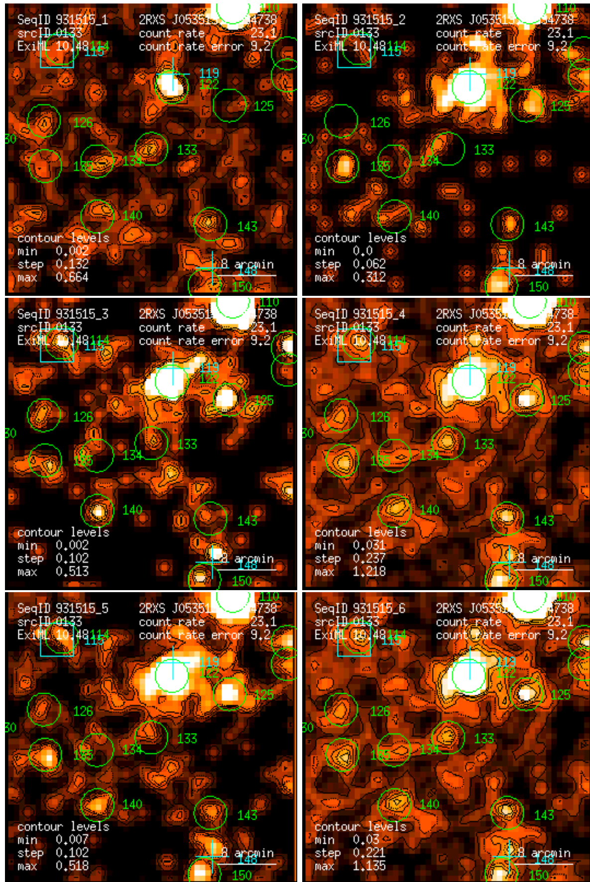
Figure 133: RASS 931515: detection 0133: band rate images, Gaussian filter: (1) PSPC channels 11 – 41, (2) 52 – 90, (3) 91 – 201, (4) 11 – 235, (5) 52 – 201, (6) 11 – 201. Broad band rates in counts/ks. Band rate contour levels in counts/ks/arcmin 2 .
