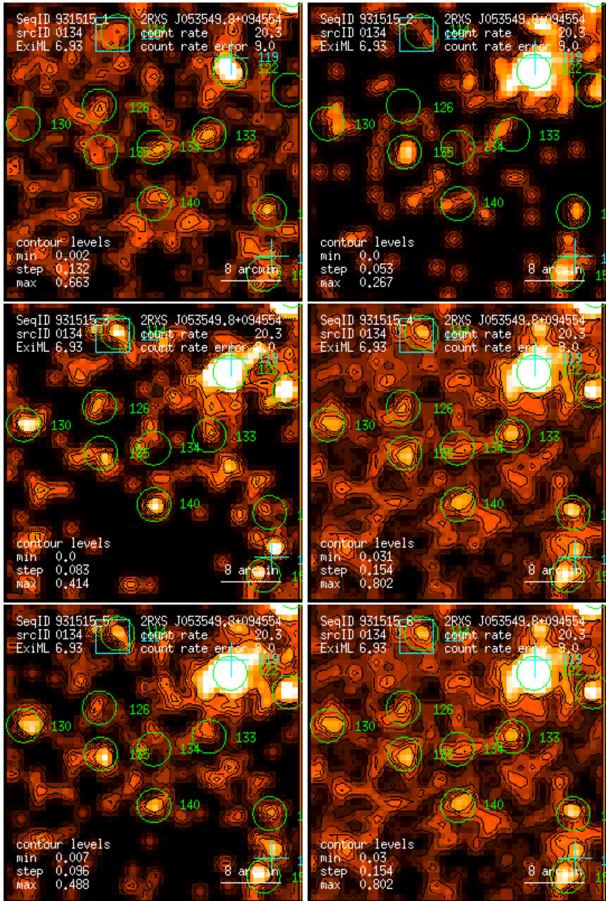
Figure 134: RASS 931515: detection 0134: band rate images, Gaussian filter: (1) PSPC channels 11 – 41, (2) 52 – 90, (3) 91 – 201, (4) 11 – 235, (5) 52 – 201, (6) 11 – 201. Broad band rates in counts/ks. Band rate contour levels in counts/ks/arcmin 2 .
