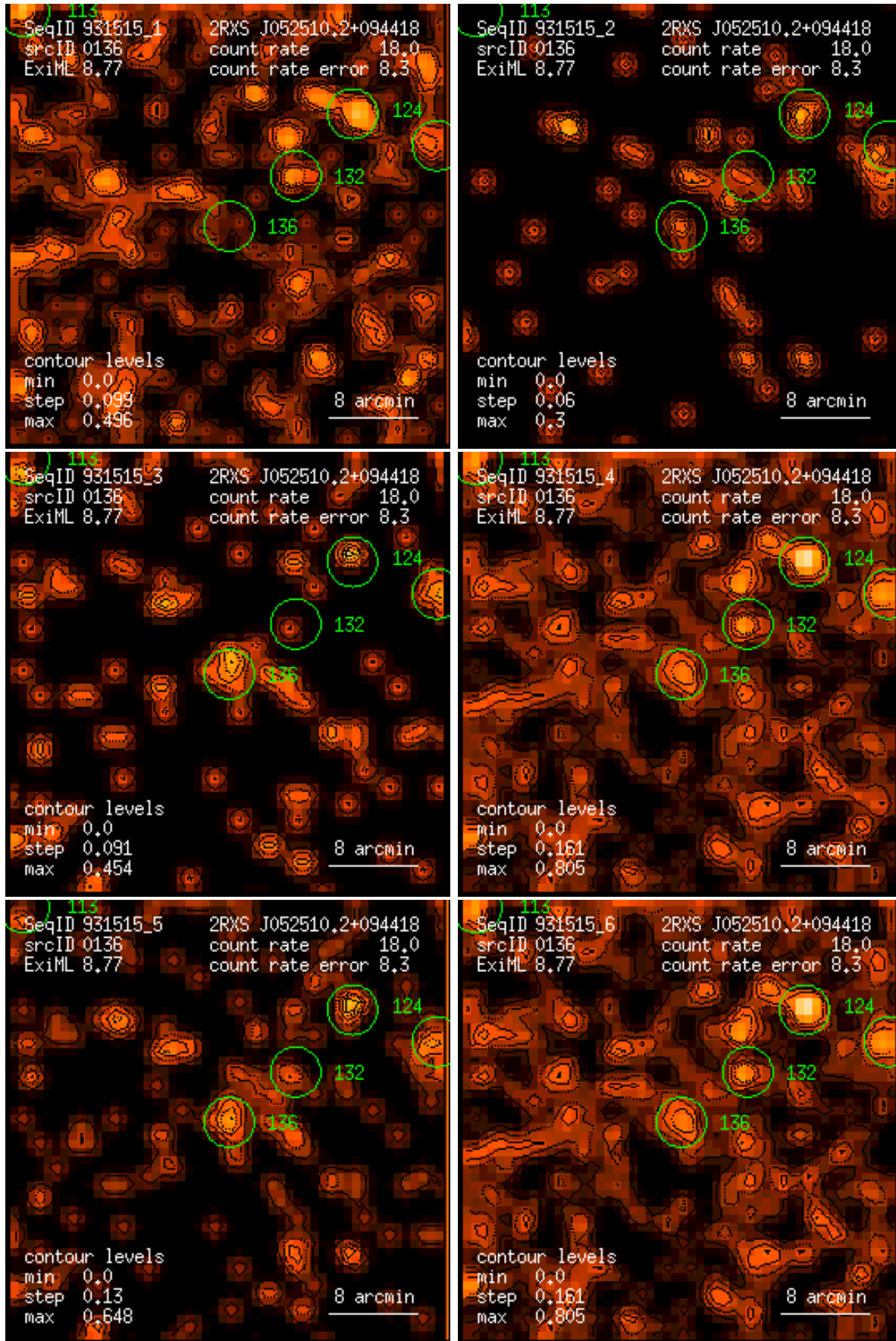
Figure 136: RASS 931515: detection 0136: band rate images, Gaussian filter: (1) PSPC channels 11 – 41, (2) 52 – 90, (3) 91 – 201, (4) 11 – 235, (5) 52 – 201, (6) 11 – 201. Broad band rates in counts/ks. Band rate contour levels in counts/ks/arcmin 2 .
