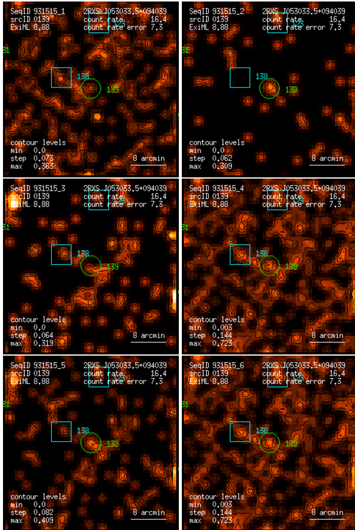
Figure 139: RASS 931515: detection 0139: band rate images, Gaussian filter: (1) PSPC channels 11 – 41, (2) 52 – 90, (3) 91 – 201, (4) 11 – 235, (5) 52 – 201, (6) 11 – 201. Broad band rates in counts/ks. Band rate contour levels in counts/ks/arcmin 2 .
