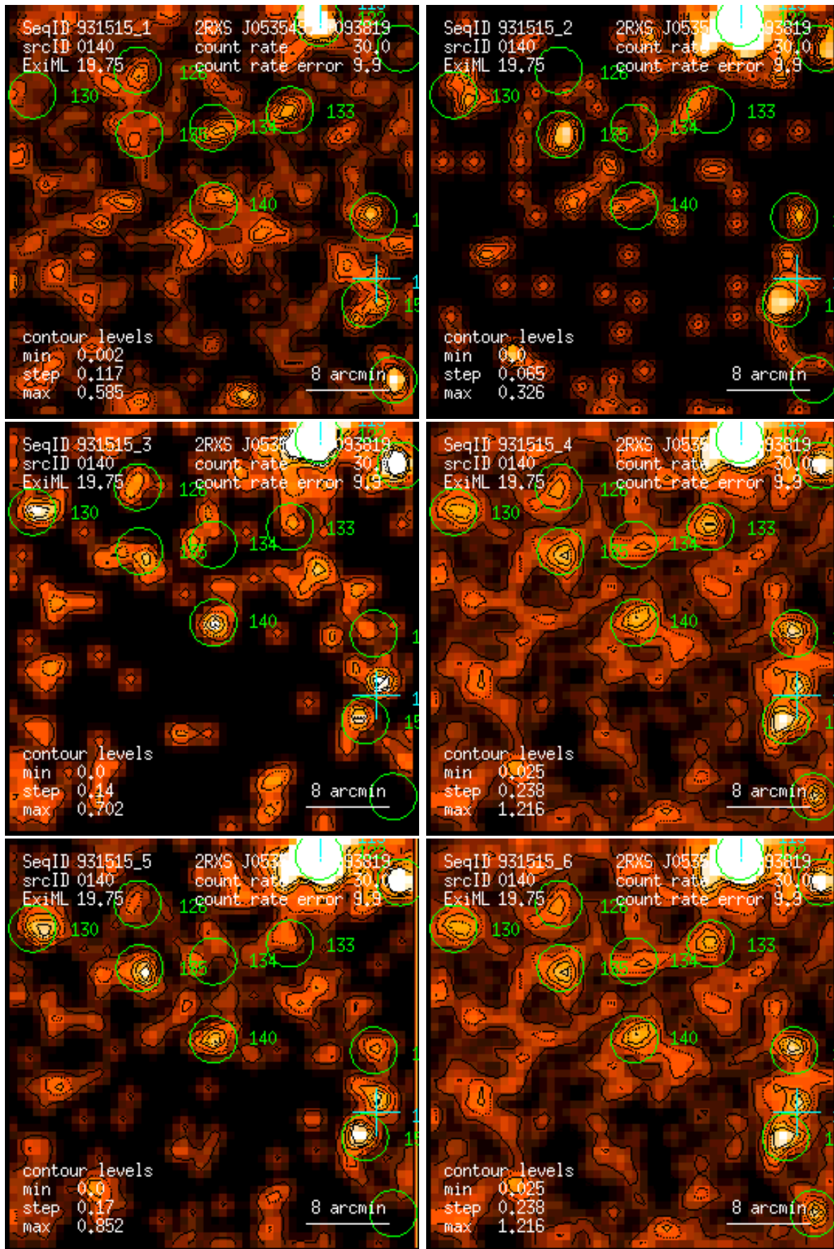
Figure 140: RASS 931515: detection 0140: band rate images, Gaussian filter: (1) PSPC channels 11 – 41, (2) 52 – 90, (3) 91 – 201, (4) 11 – 235, (5) 52 – 201, (6) 11 – 201. Broad band rates in counts/ks. Band rate contour levels in counts/ks/arcmin 2 .
