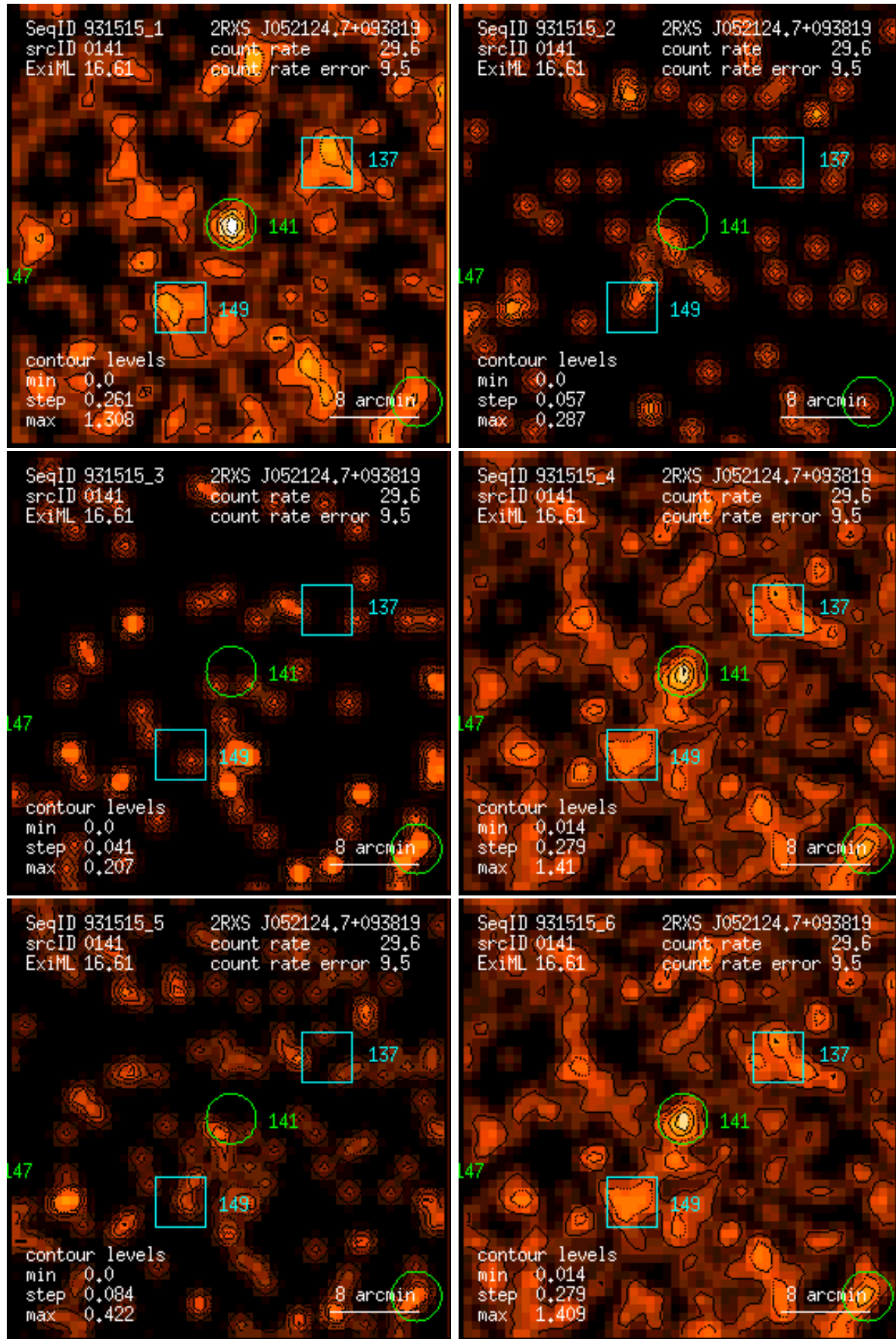
Figure 141: RASS 931515: detection 0141: band rate images, Gaussian filter: (1) PSPC channels 11 – 41, (2) 52 – 90, (3) 91 – 201, (4) 11 – 235, (5) 52 – 201, (6) 11 – 201. Broad band rates in counts/ks. Band rate contour levels in counts/ks/arcmin 2 .
