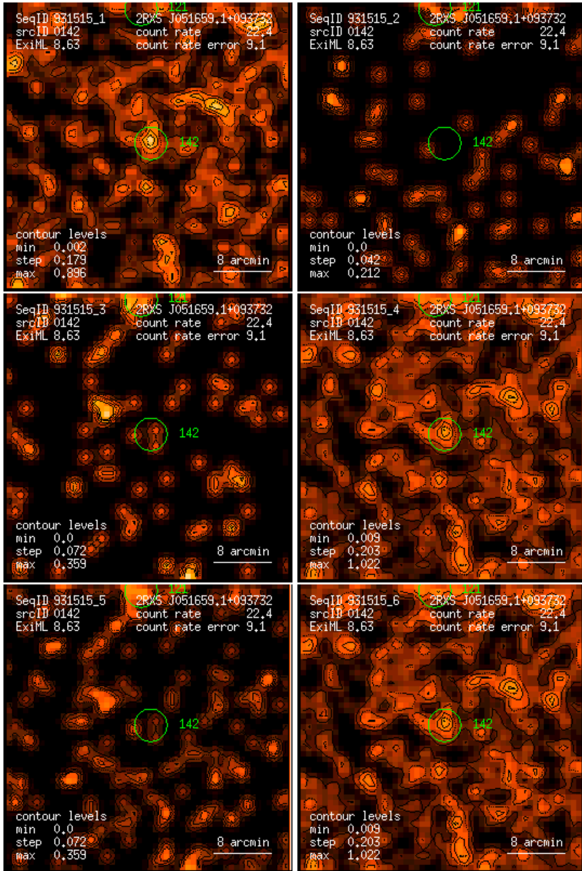
Figure 142: RASS 931515: detection 0142: band rate images, Gaussian filter: (1) PSPC channels 11 – 41, (2) 52 – 90, (3) 91 – 201, (4) 11 – 235, (5) 52 – 201, (6) 11 – 201. Broad band rates in counts/ks. Band rate contour levels in counts/ks/arcmin 2 .
