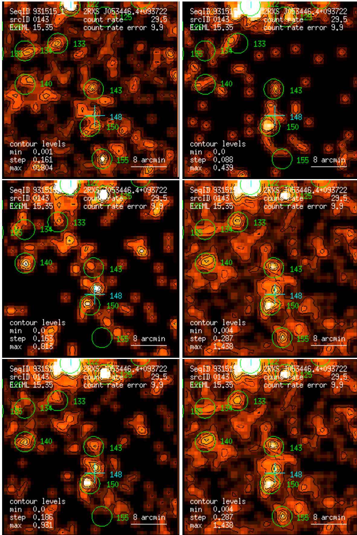
Figure 143: RASS 931515: detection 0143: band rate images, Gaussian filter: (1) PSPC channels 11 – 41, (2) 52 – 90, (3) 91 – 201, (4) 11 – 235, (5) 52 – 201, (6) 11 – 201. Broad band rates in counts/ks. Band rate contour levels in counts/ks/arcmin 2 .
