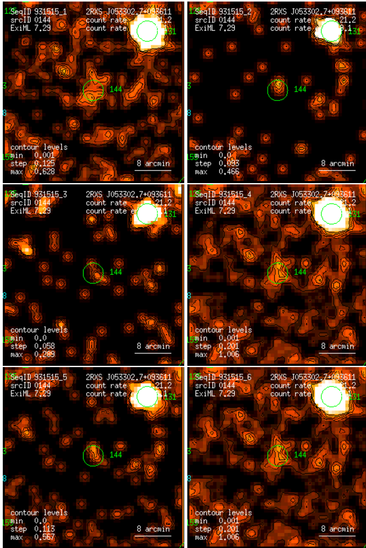
Figure 144: RASS 931515: detection 0144: band rate images, Gaussian filter: (1) PSPC channels 11 – 41, (2) 52 – 90, (3) 91 – 201, (4) 11 – 235, (5) 52 – 201, (6) 11 – 201. Broad band rates in counts/ks. Band rate contour levels in counts/ks/arcmin 2 .
