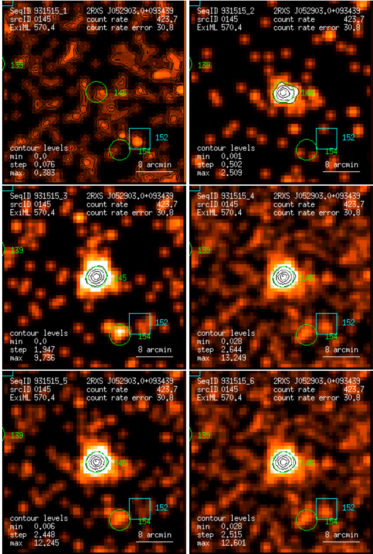
Figure 145: RASS 931515: detection 0145: band rate images, Gaussian filter: (1) PSPC channels 11 – 41, (2) 52 – 90, (3) 91 – 201, (4) 11 – 235, (5) 52 – 201, (6) 11 – 201. Broad band rates in counts/ks. Band rate contour levels in counts/ks/arcmin 2 .
