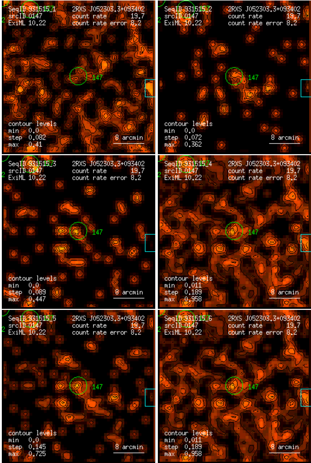
Figure 147: RASS 931515: detection 0147: band rate images, Gaussian filter: (1) PSPC channels 11 – 41, (2) 52 – 90, (3) 91 – 201, (4) 11 – 235, (5) 52 – 201, (6) 11 – 201. Broad band rates in counts/ks. Band rate contour levels in counts/ks/arcmin 2 .
