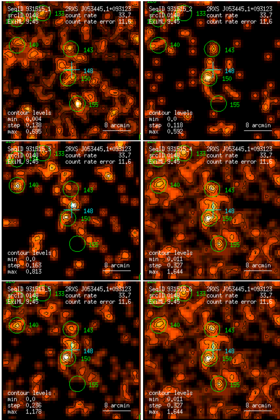
Figure 148: RASS 931515: detection 0148: band rate images, Gaussian filter: (1) PSPC channels 11 – 41, (2) 52 – 90, (3) 91 – 201, (4) 11 – 235, (5) 52 – 201, (6) 11 – 201. Broad band rates in counts/ks. Band rate contour levels in counts/ks/arcmin 2 .
