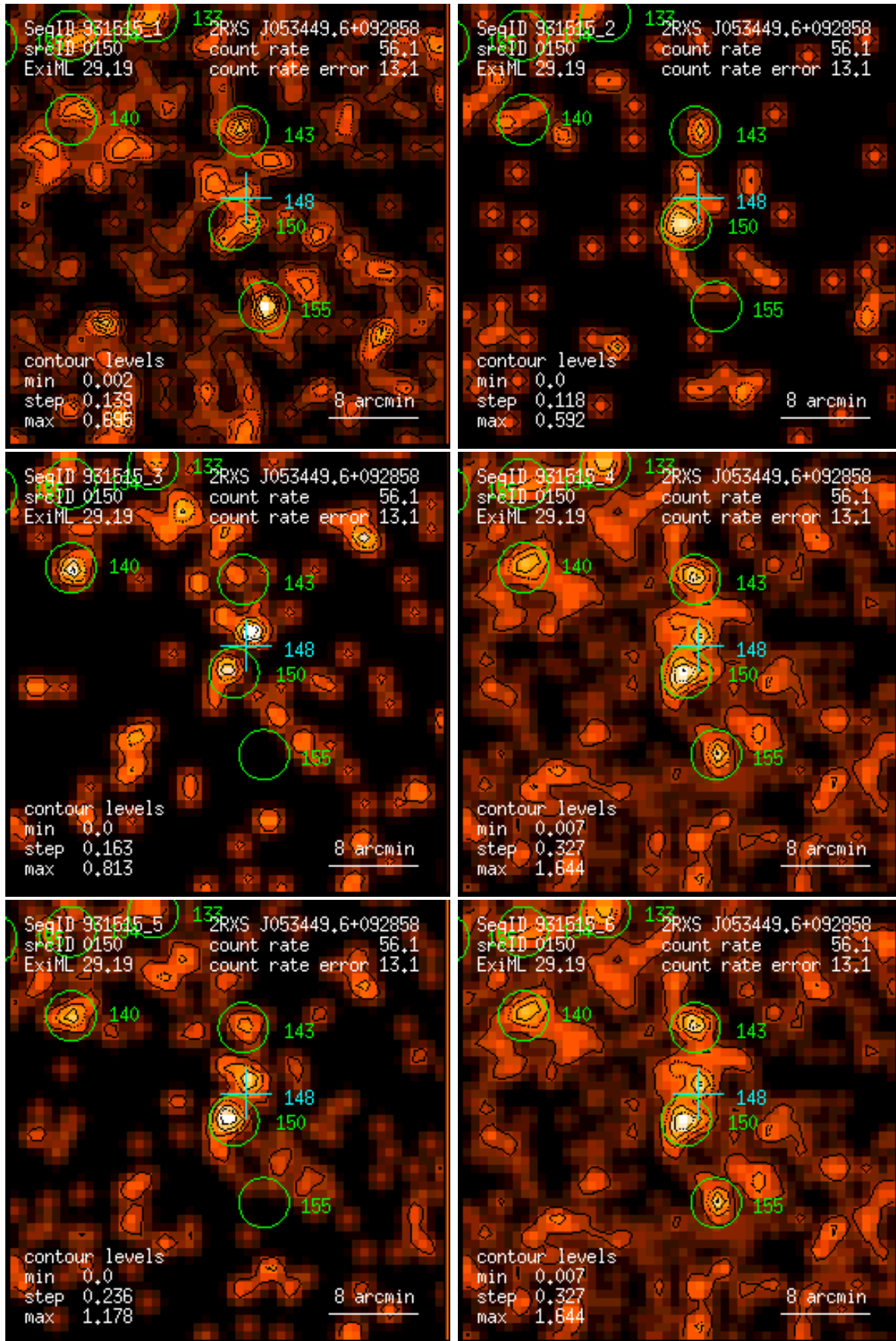
Figure 150: RASS 931515: detection 0150: band rate images, Gaussian filter: (1) PSPC channels 11 – 41, (2) 52 – 90, (3) 91 – 201, (4) 11 – 235, (5) 52 – 201, (6) 11 – 201. Broad band rates in counts/ks. Band rate contour levels in counts/ks/arcmin 2 .
