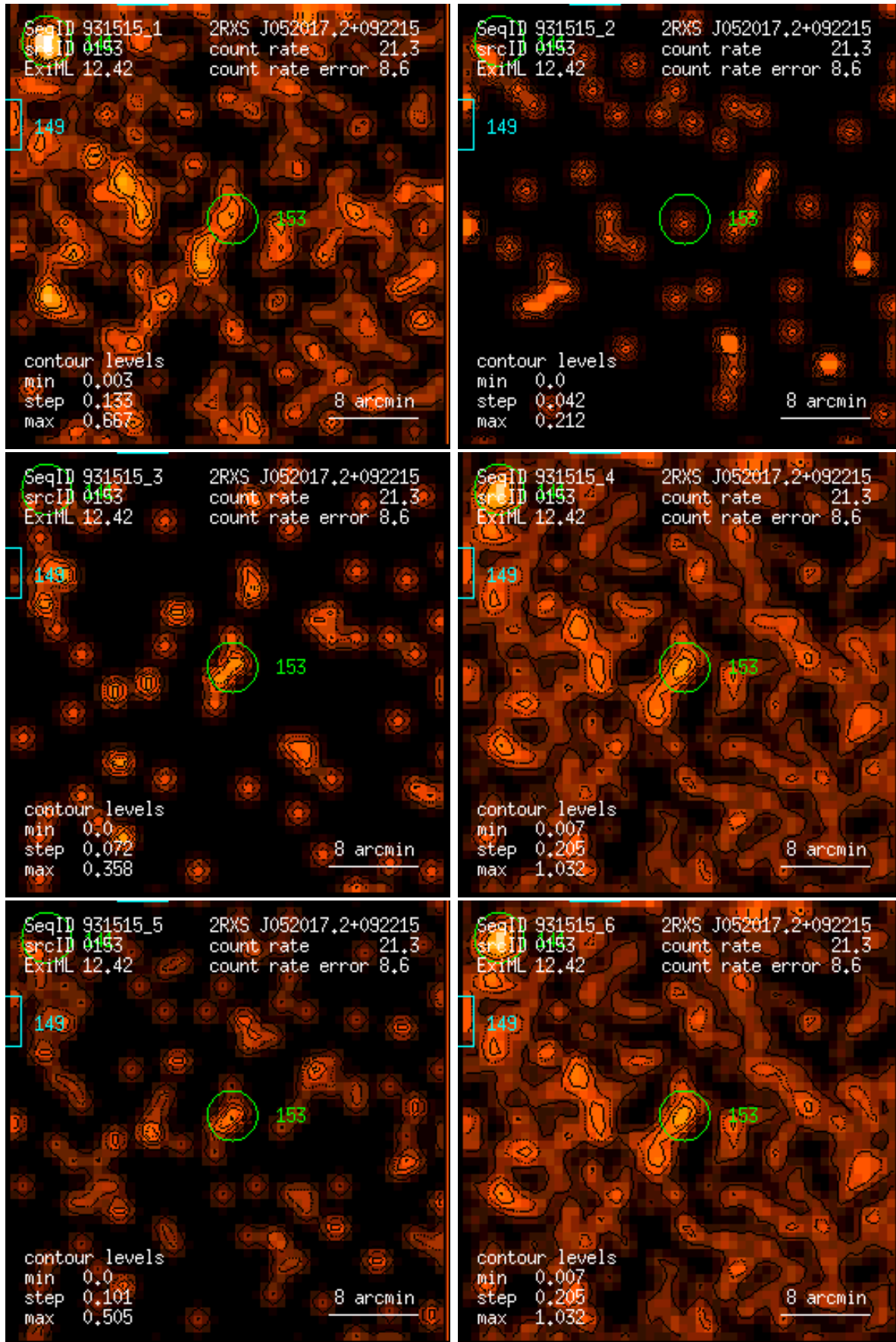
Figure 153: RASS 931515: detection 0153: band rate images, Gaussian filter: (1) PSPC channels 11 – 41, (2) 52 – 90, (3) 91 – 201, (4) 11 – 235, (5) 52 – 201, (6) 11 – 201. Broad band rates in counts/ks. Band rate contour levels in counts/ks/arcmin 2 .
