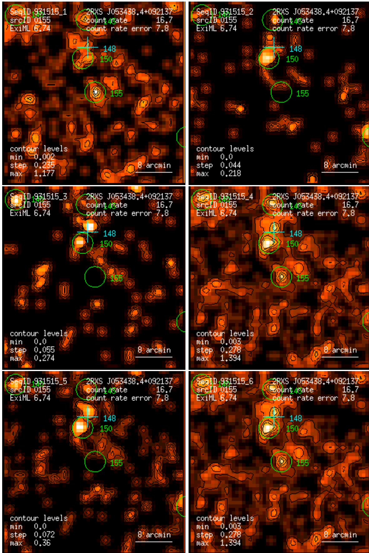
Figure 155: RASS 931515: detection 0155: band rate images, Gaussian filter: (1) PSPC channels 11 – 41, (2) 52 – 90, (3) 91 – 201, (4) 11 – 235, (5) 52 – 201, (6) 11 – 201. Broad band rates in counts/ks. Band rate contour levels in counts/ks/arcmin 2 .
