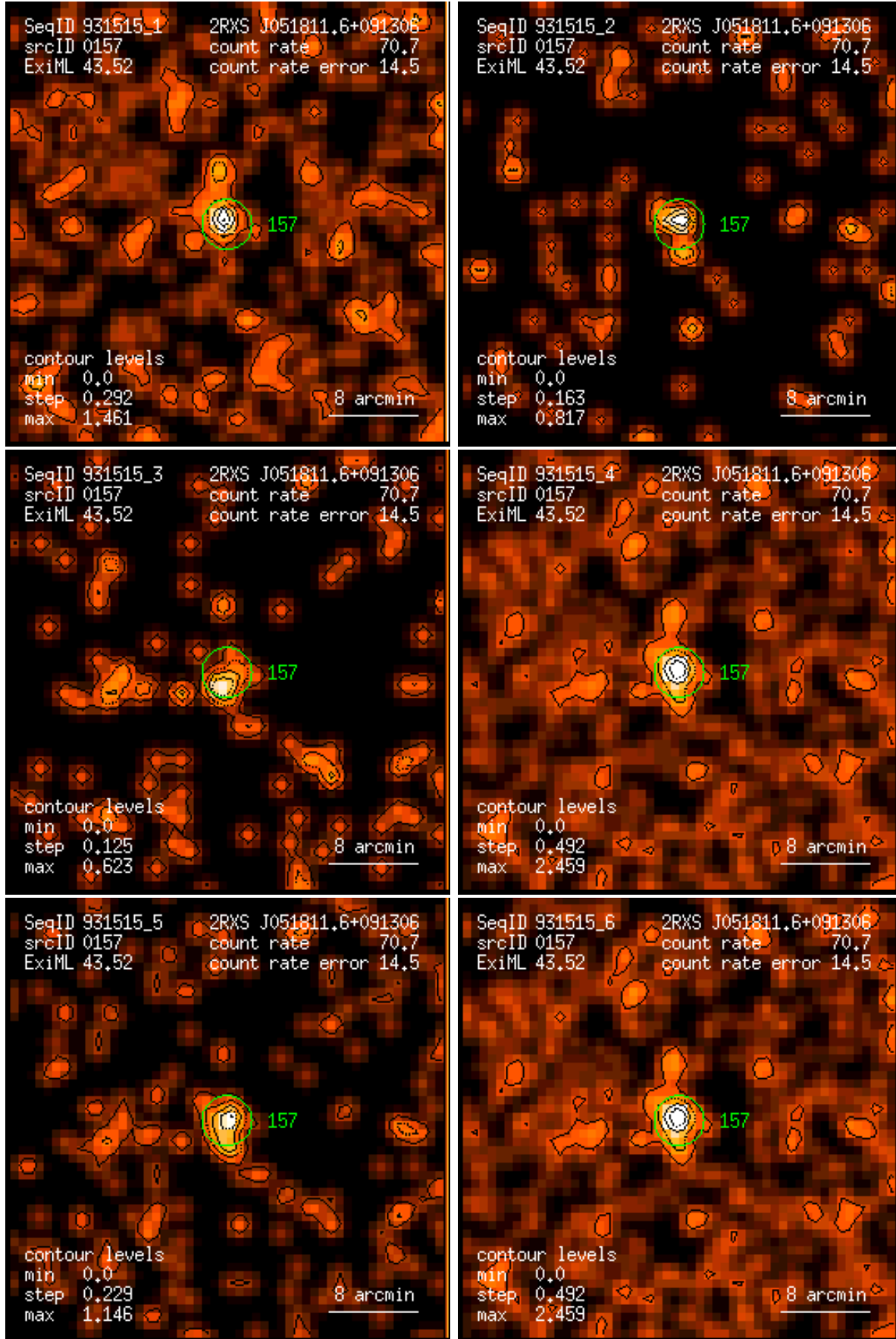
Figure 157: RASS 931515: detection 0157: band rate images, Gaussian filter: (1) PSPC channels 11 – 41, (2) 52 – 90, (3) 91 – 201, (4) 11 – 235, (5) 52 – 201, (6) 11 – 201. Broad band rates in counts/ks. Band rate contour levels in counts/ks/arcmin 2 .
