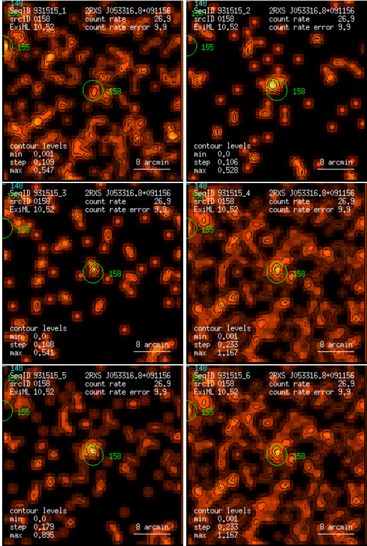
Figure 158: RASS 931515: detection 0158: band rate images, Gaussian filter: (1) PSPC channels 11 – 41, (2) 52 – 90, (3) 91 – 201, (4) 11 – 235, (5) 52 – 201, (6) 11 – 201. Broad band rates in counts/ks. Band rate contour levels in counts/ks/arcmin 2 .
