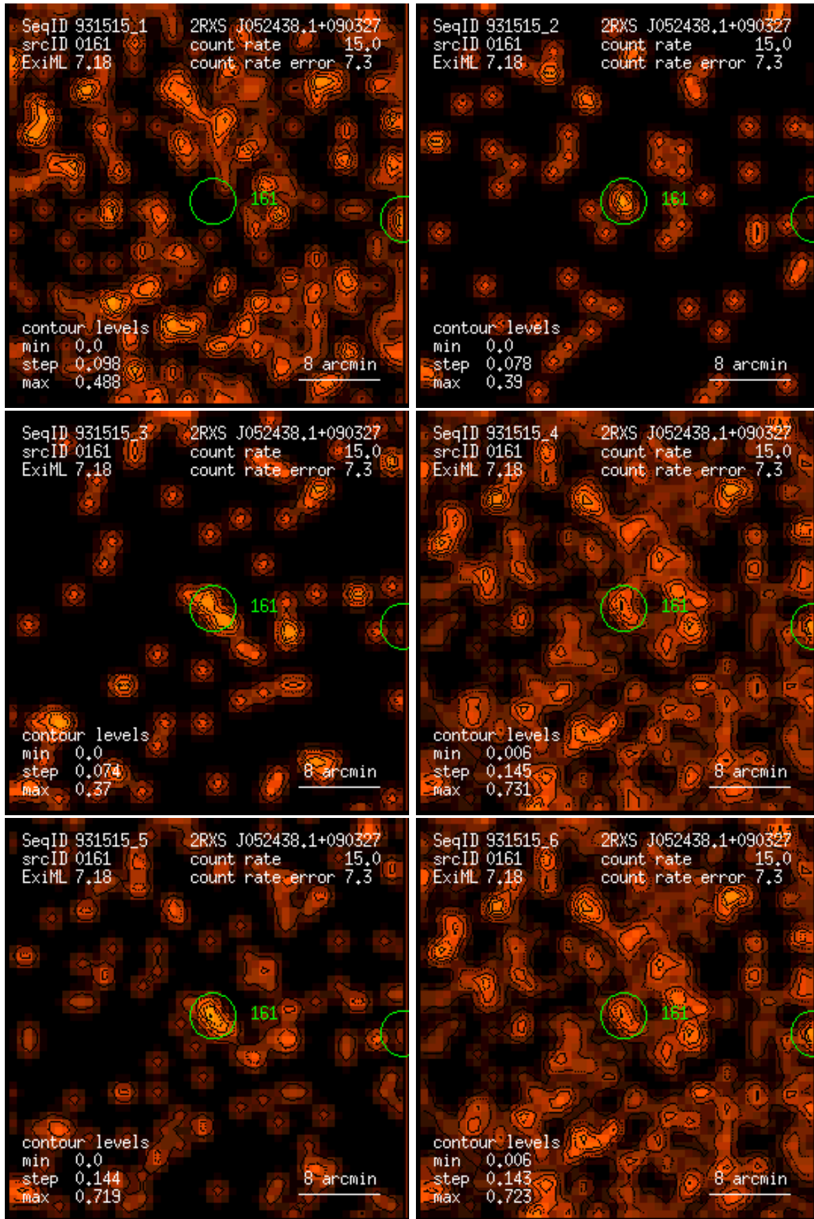
Figure 161: RASS 931515: detection 0161: band rate images, Gaussian filter: (1) PSPC channels 11 – 41, (2) 52 – 90, (3) 91 – 201, (4) 11 – 235, (5) 52 – 201, (6) 11 – 201. Broad band rates in counts/ks. Band rate contour levels in counts/ks/arcmin 2 .
