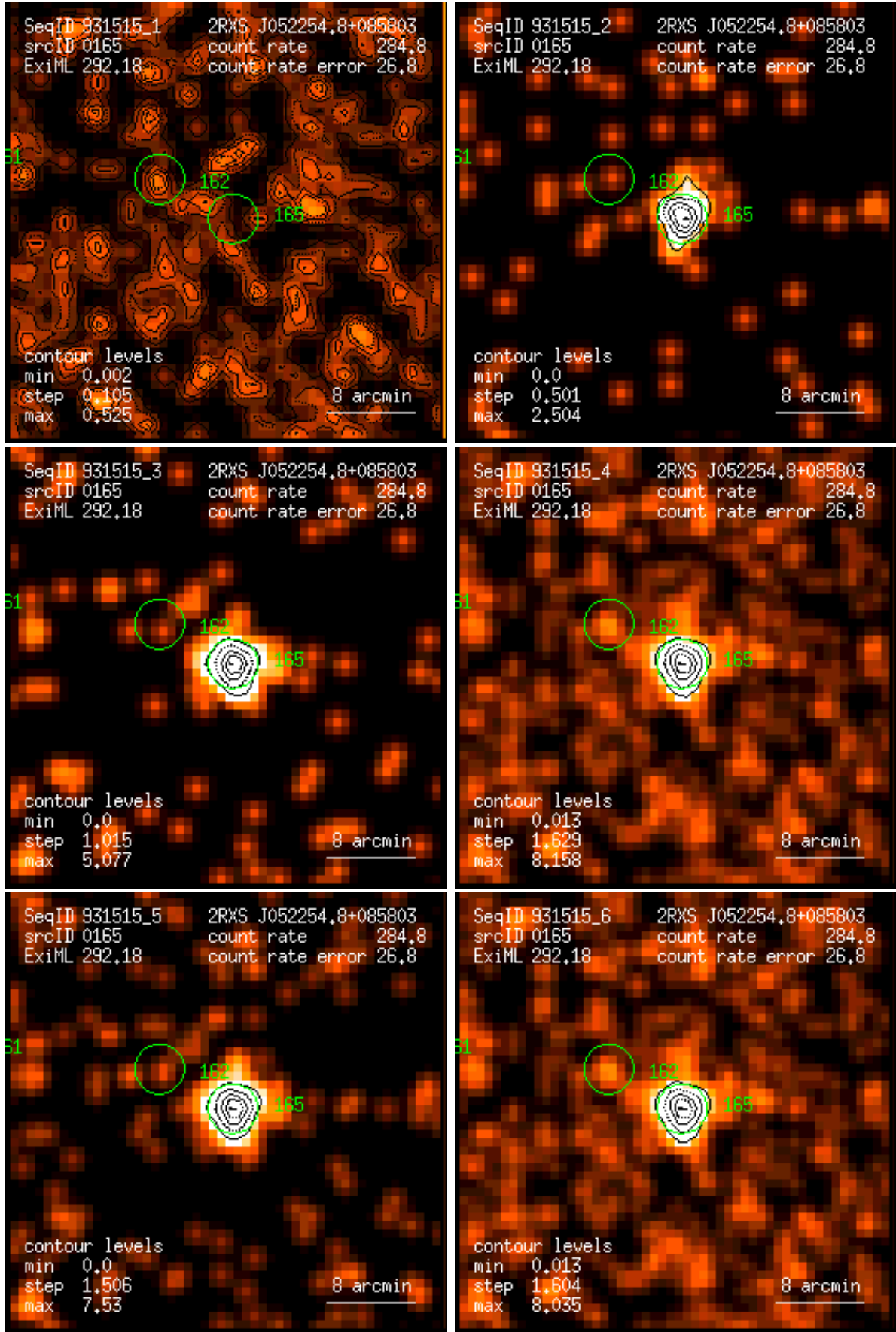
Figure 165: RASS 931515: detection 0165: band rate images, Gaussian filter: (1) PSPC channels 11 – 41, (2) 52 – 90, (3) 91 – 201, (4) 11 – 235, (5) 52 – 201, (6) 11 – 201. Broad band rates in counts/ks. Band rate contour levels in counts/ks/arcmin 2 .
