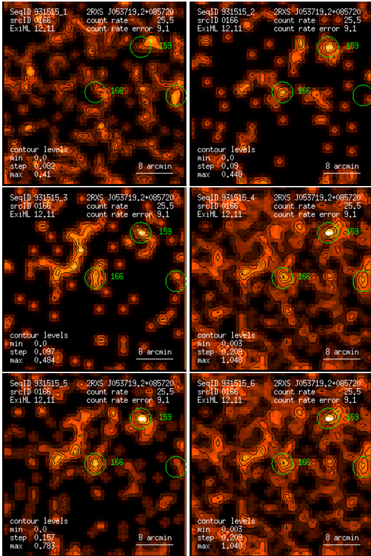
Figure 166: RASS 931515: detection 0166: band rate images, Gaussian filter: (1) PSPC channels 11 – 41, (2) 52 – 90, (3) 91 – 201, (4) 11 – 235, (5) 52 – 201, (6) 11 – 201. Broad band rates in counts/ks. Band rate contour levels in counts/ks/arcmin 2 .
