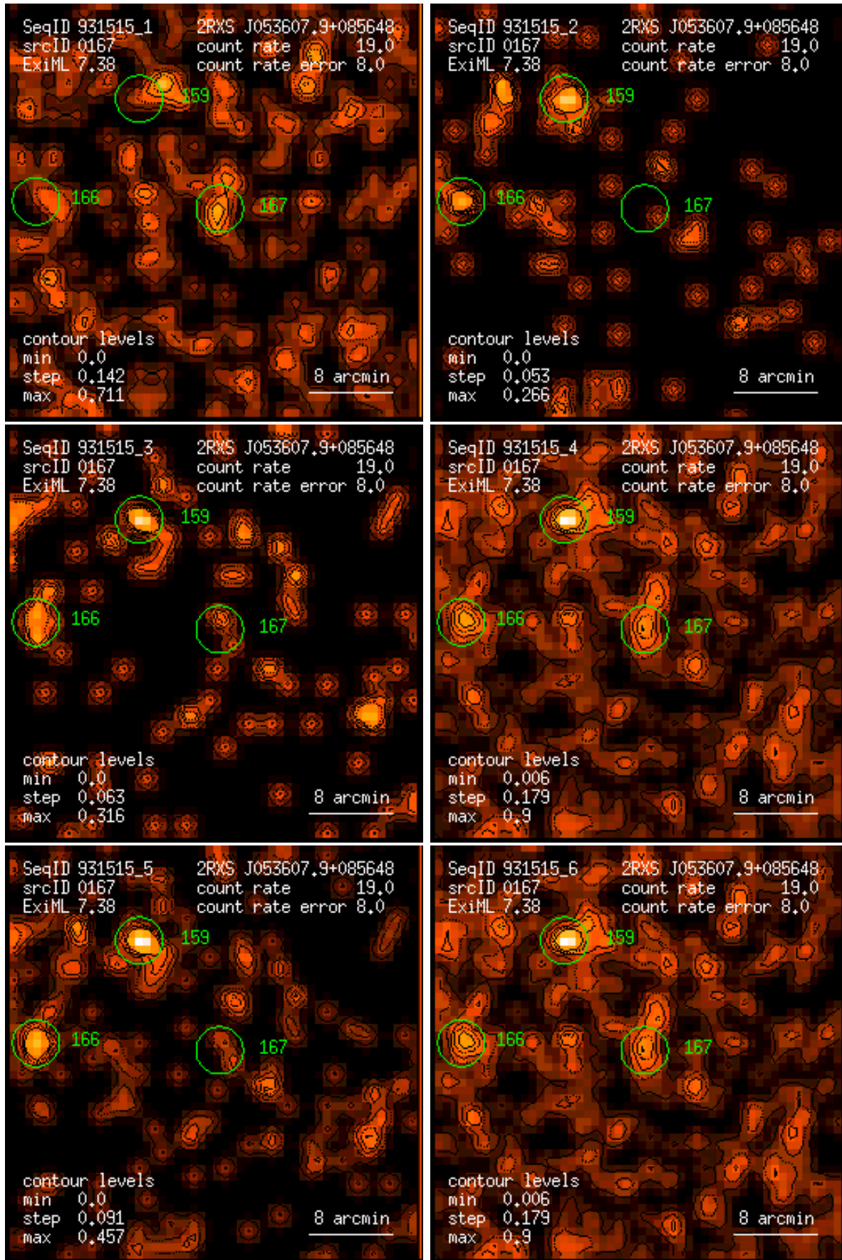
Figure 167: RASS 931515: detection 0167: band rate images, Gaussian filter: (1) PSPC channels 11 – 41, (2) 52 – 90, (3) 91 – 201, (4) 11 – 235, (5) 52 – 201, (6) 11 – 201. Broad band rates in counts/ks. Band rate contour levels in counts/ks/arcmin 2 .
