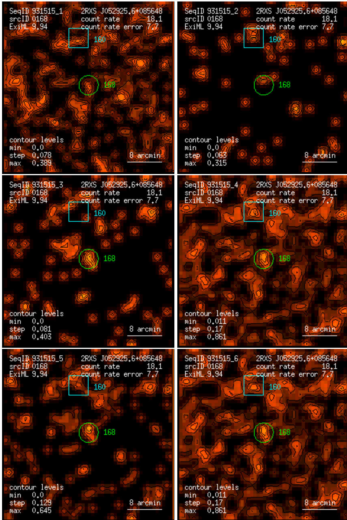
Figure 168: RASS 931515: detection 0168: band rate images, Gaussian filter: (1) PSPC channels 11 – 41, (2) 52 – 90, (3) 91 – 201, (4) 11 – 235, (5) 52 – 201, (6) 11 – 201. Broad band rates in counts/ks. Band rate contour levels in counts/ks/arcmin 2 .
