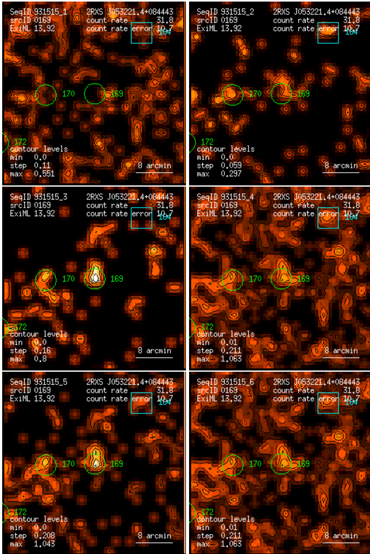
Figure 169: RASS 931515: detection 0169: band rate images, Gaussian filter: (1) PSPC channels 11 – 41, (2) 52 – 90, (3) 91 – 201, (4) 11 – 235, (5) 52 – 201, (6) 11 – 201. Broad band rates in counts/ks. Band rate contour levels in counts/ks/arcmin 2 .
