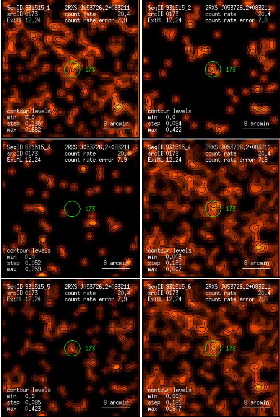
Figure 173: RASS 931515: detection 0173: band rate images, Gaussian filter: (1) PSPC channels 11 – 41, (2) 52 – 90, (3) 91 – 201, (4) 11 – 235, (5) 52 – 201, (6) 11 – 201. Broad band rates in counts/ks. Band rate contour levels in counts/ks/arcmin 2 .
