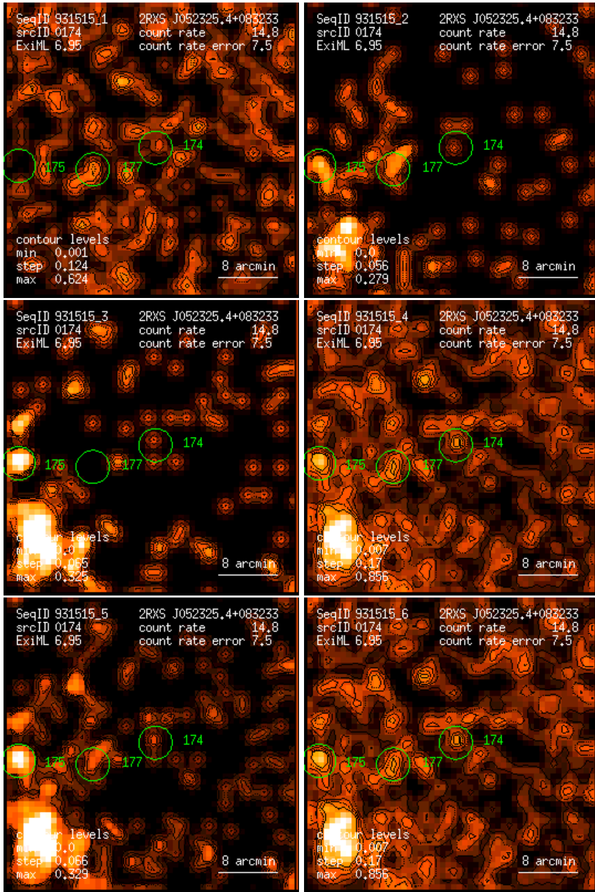
Figure 174: RASS 931515: detection 0174: band rate images, Gaussian filter: (1) PSPC channels 11 – 41, (2) 52 – 90, (3) 91 – 201, (4) 11 – 235, (5) 52 – 201, (6) 11 – 201. Broad band rates in counts/ks. Band rate contour levels in counts/ks/arcmin 2 .
