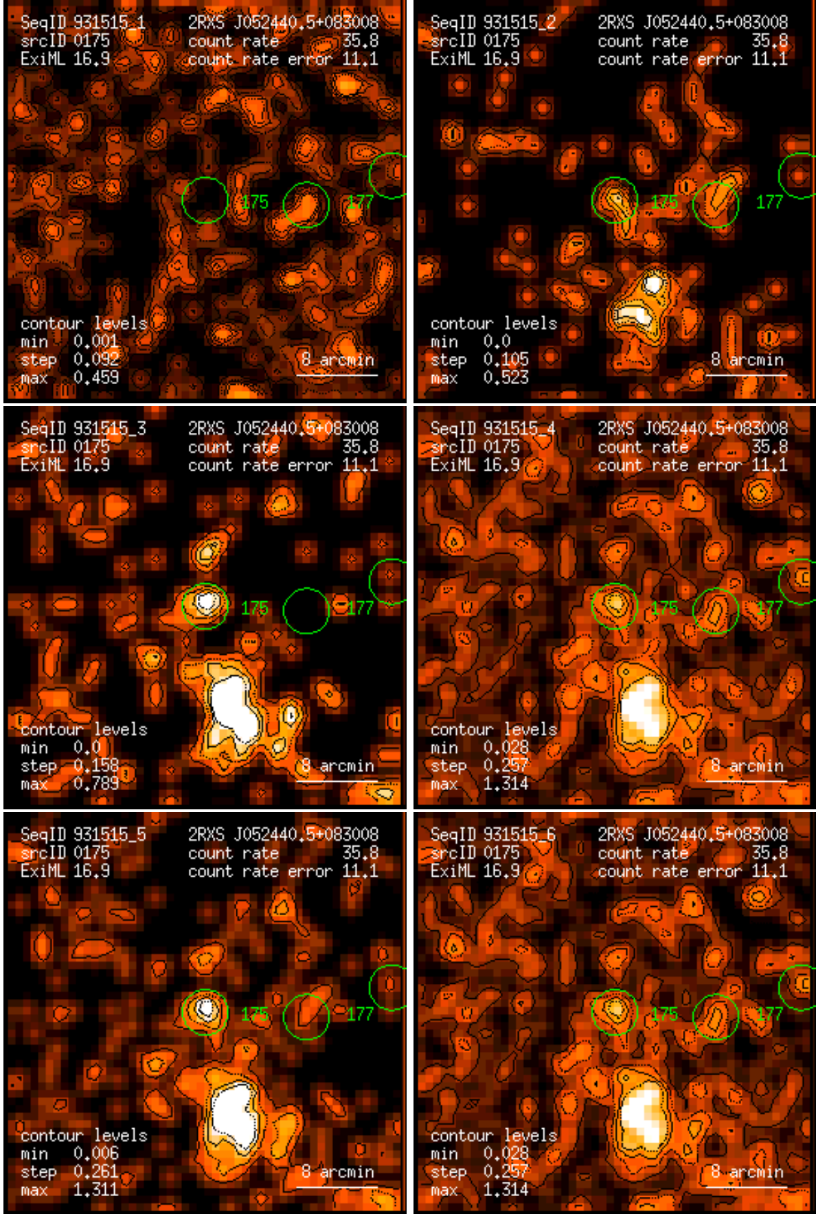
Figure 175: RASS 931515: detection 0175: band rate images, Gaussian filter: (1) PSPC channels 11 – 41, (2) 52 – 90, (3) 91 – 201, (4) 11 – 235, (5) 52 – 201, (6) 11 – 201. Broad band rates in counts/ks. Band rate contour levels in counts/ks/arcmin 2 .
